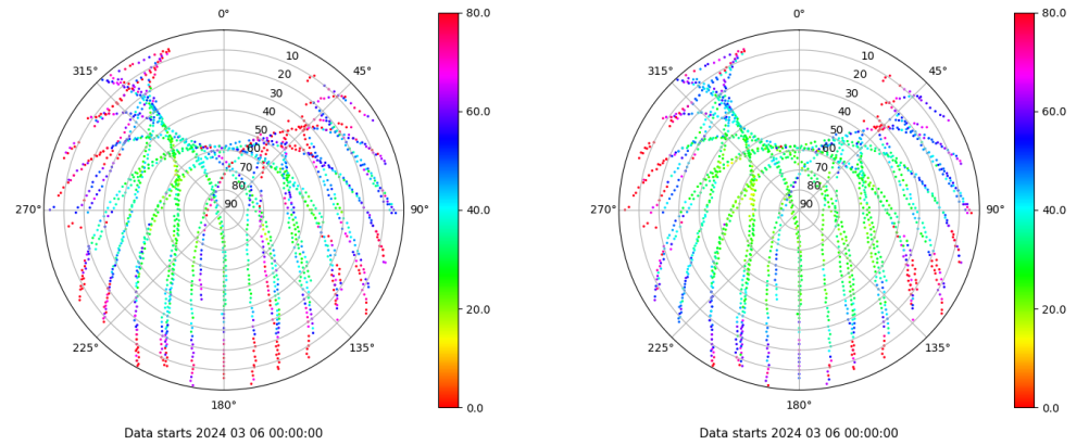
Skyplot for station ALC1. Parameter M1C Data file ALC100ESP_R_2024066.xtr Skyplot for station ALC1. Parameter M2C Data file ALC100ESP_R_2024066.xtr
