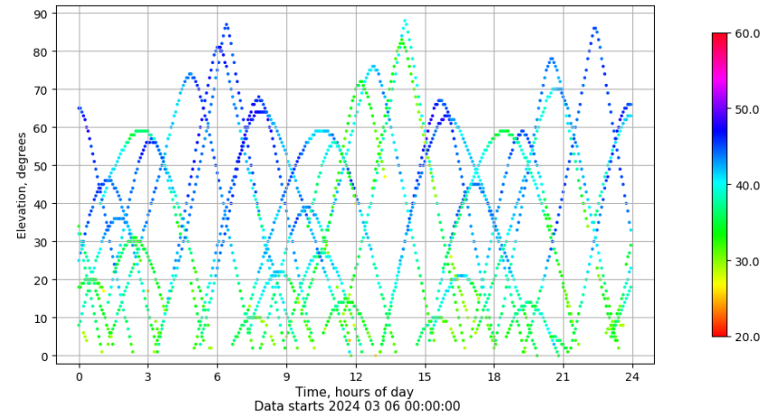
Time-elevation plot for station ALC1. Signal to Noise S1C Data file ALC100ESP_R_2024066.xtr
