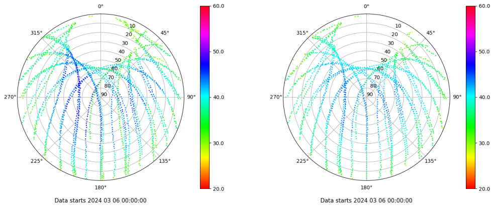
Skyplot for station ALC1. Signal to Noise S1C Data file ALC100ESP_R_2024066.xtr Skyplot for station ALC1. Signal to Noise S2C Data file ALC100ESP_R_2024066.xtr
