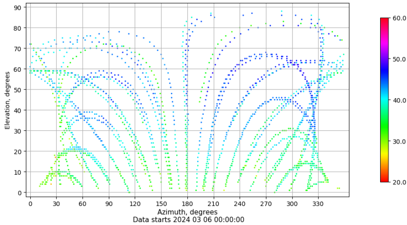
Azimuth-elevation plot for station ALC1. Signal to Noise S1C Data file ALC100ESP_R_2024066.xtr
