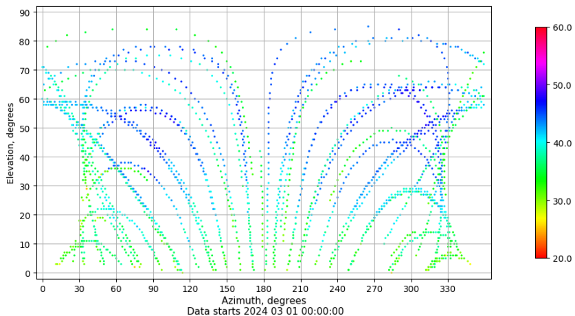
Azimuth-elevation plot for station ALC1. Signal to Noise S1C Data file ALC100ESP_R_2024061.xtr
