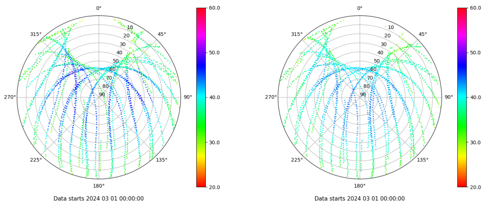
Skyplot for station ALC1. Signal to Noise S1C Data file ALC100ESP_R_2024061.xtr Skyplot for station ALC1. Signal to Noise S2C Data file ALC100ESP_R_2024061.xtr
