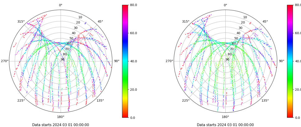
Skyplot for station ALC1. Parameter M1C Data file ALC100ESP_R_2024061.xtr Skyplot for station ALC1. Parameter M2C Data file ALC100ESP_R_2024061.xtr
