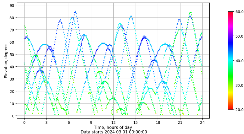
Time-elevation plot for station ALC1. Signal to Noise S1C Data file ALC100ESP_R_2024061.xtr
