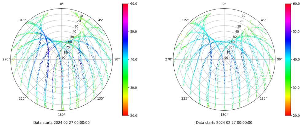
Skyplot for station ALC1. Signal to Noise S1C Data file ALC100ESP_R_2024058.xtr Skyplot for station ALC1. Signal to Noise S2C Data file ALC100ESP_R_2024058.xtr
