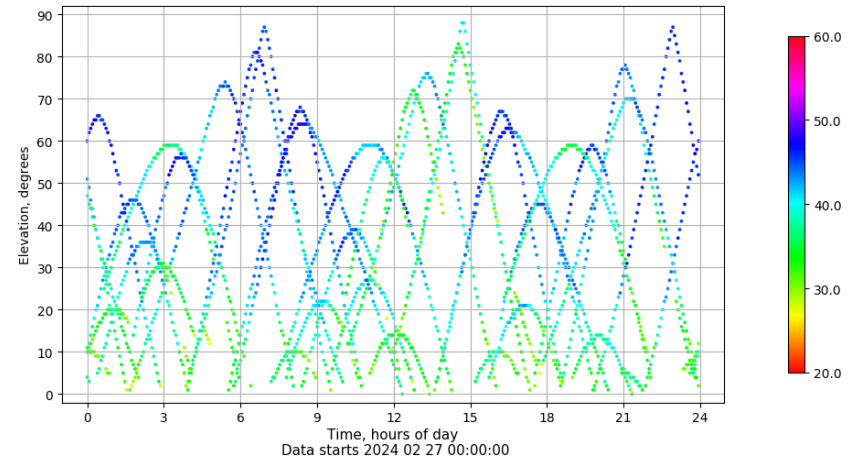
Time-elevation plot for station ALC1. Signal to Noise S1C Data file ALC100ESP_R_2024058.xtr
