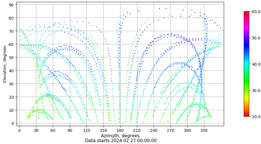
Azimuth-elevation plot for station ALC1. Signal to Noise S1C Data file ALC100ESP_R_2024058.xtr
