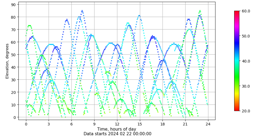
Time-elevation plot for station ALC1. Signal to Noise S1C Data file ALC100ESP_R_2024053.xtr
