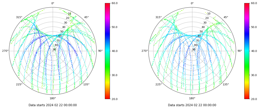
Skyplot for station ALC1. Signal to Noise S1C Data file ALC100ESP_R_2024053.xtr Skyplot for station ALC1. Signal to Noise S2C Data file ALC100ESP_R_2024053.xtr
