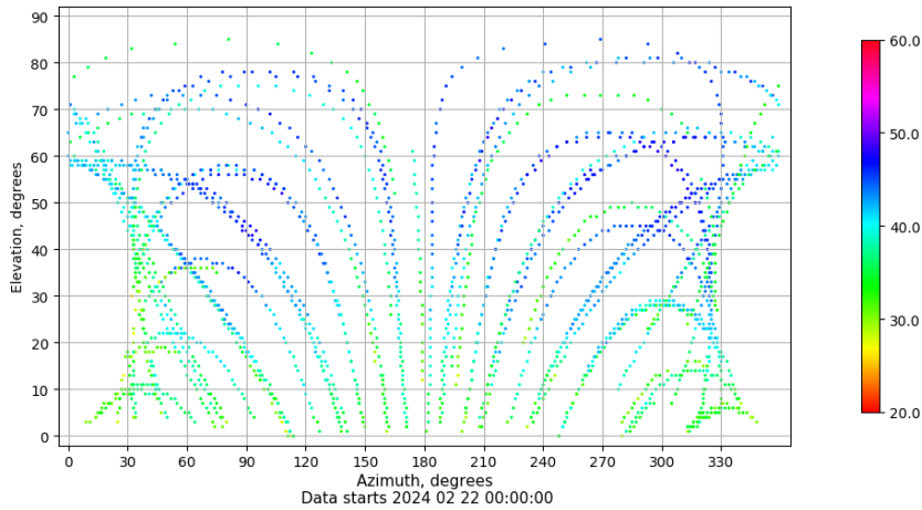
Azimuth-elevation plot for station ALC1. Signal to Noise S1C Data file ALC100ESP_R_2024053.xtr
