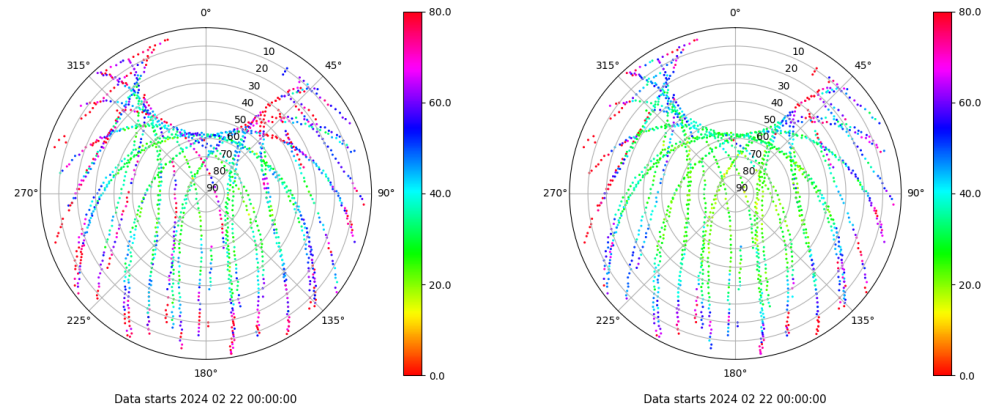
Skyplot for station ALC1. Parameter M1C Data file ALC100ESP_R_2024053.xtr Skyplot for station ALC1. Parameter M2C Data file ALC100ESP_R_2024053.xtr
