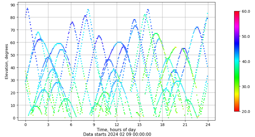
Time-elevation plot for station ALC1. Signal to Noise S1C Data file ALC100ESP_R_2024040.xtr
