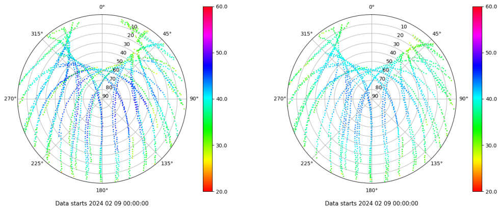
Skyplot for station ALC1. Signal to Noise S1C Data file ALC100ESP_R_2024040.xtr Skyplot for station ALC1. Signal to Noise S2C Data file ALC100ESP_R_2024040.xtr
