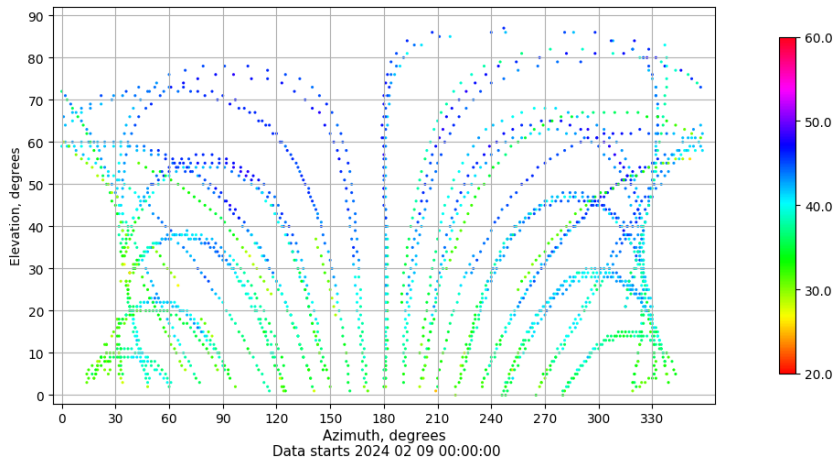
Azimuth-elevation plot for station ALC1. Signal to Noise S1C Data file ALC100ESP_R_2024040.xtr
