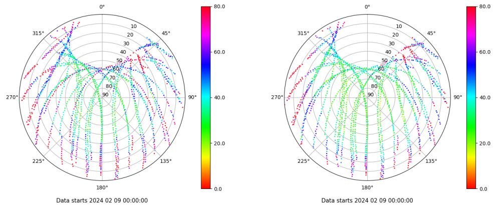
Skyplot for station ALC1. Parameter M1C Data file ALC100ESP_R_2024040.xtr Skyplot for station ALC1. Parameter M2C Data file ALC100ESP_R_2024040.xtr
