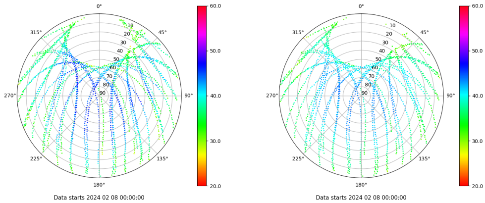
Skyplot for station ALC1. Signal to Noise S1C Data file ALC100ESP_R_2024039.xtr Skyplot for station ALC1. Signal to Noise S2C Data file ALC100ESP_R_2024039.xtr
