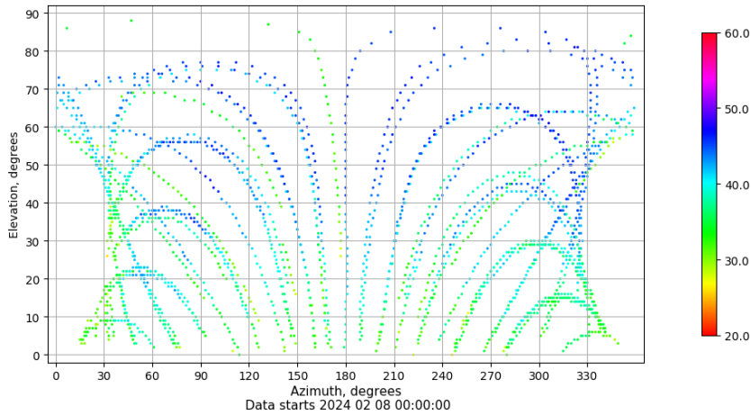
Azimuth-elevation plot for station ALC1. Signal to Noise S1C Data file ALC100ESP_R_2024039.xtr
