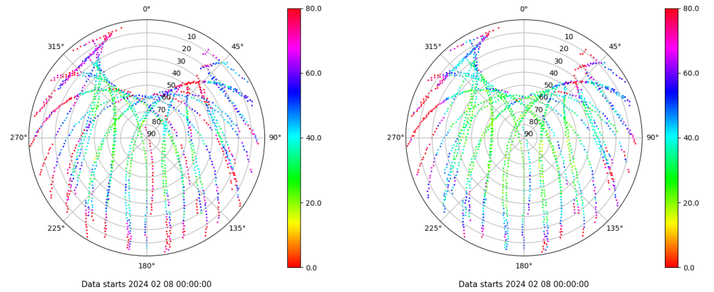
Skyplot for station ALC1. Parameter M1C Data file ALC100ESP_R_2024039.xtr Skyplot for station ALC1. Parameter M2C Data file ALC100ESP_R_2024039.xtr
