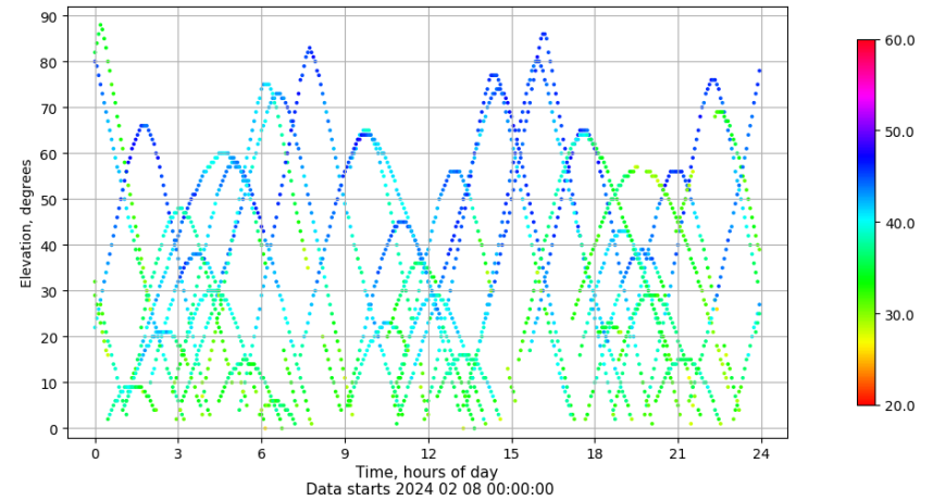
Time-elevation plot for station ALC1. Signal to Noise S1C Data file ALC100ESP_R_2024039.xtr
