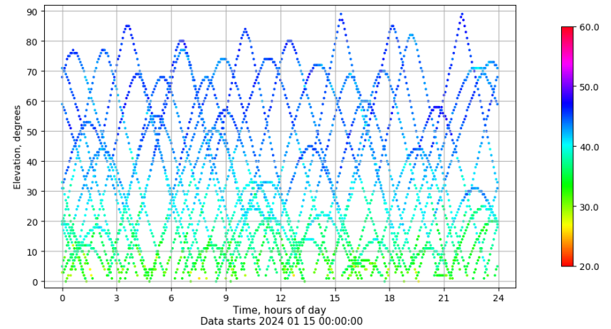
Time-elevation plot for station ALC1. Signal to Noise S1C Data file ALC100ESP_R_2024015.xtr
