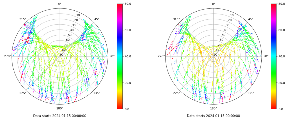
Skyplot for station ALC1. Parameter M1C Data file ALC100ESP_R_2024015.xtr Skyplot for station ALC1. Parameter M2X Data file ALC100ESP_R_2024015.xtr
