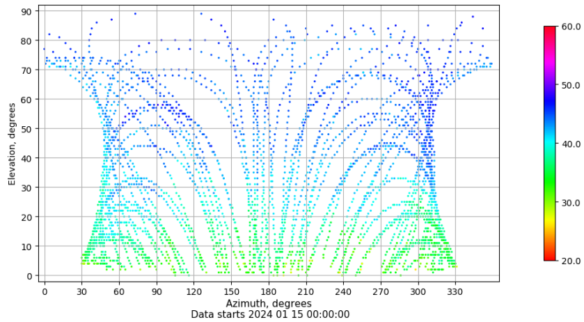
Azimuth-elevation plot for station ALC1. Signal to Noise S1C Data file ALC100ESP_R_2024015.xtr
