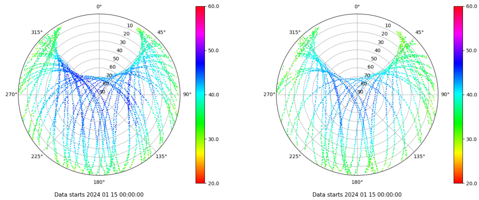
Skyplot for station ALC1. Signal to Noise S1C Data file ALC100ESP_R_2024015.xtr Skyplot for station ALC1. Signal to Noise S2X Data file ALC100ESP_R_2024015.xtr
