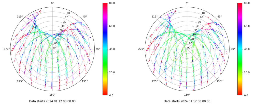
Skyplot for station ALC1. Parameter M1C Data file ALC100ESP_R_2024012.xtr Skyplot for station ALC1. Parameter M2C Data file ALC100ESP_R_2024012.xtr
