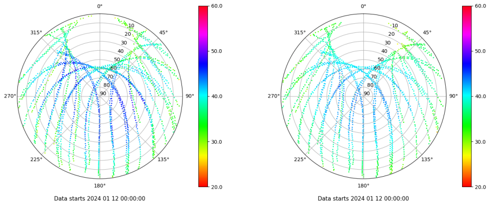
Skyplot for station ALC1. Signal to Noise S1C Data file ALC100ESP_R_2024012.xtr Skyplot for station ALC1. Signal to Noise S2C Data file ALC100ESP_R_2024012.xtr
