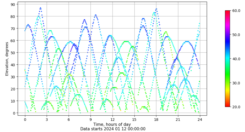
Time-elevation plot for station ALC1. Signal to Noise S1C Data file ALC100ESP_R_2024012.xtr
