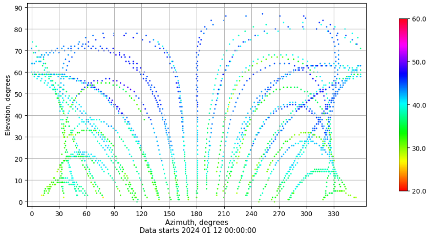
Azimuth-elevation plot for station ALC1. Signal to Noise S1C Data file ALC100ESP_R_2024012.xtr
