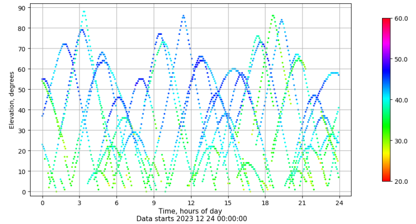
Time-elevation plot for station ALC1. Signal to Noise S1C Data file ALC100ESP_R_2023358.xtr
