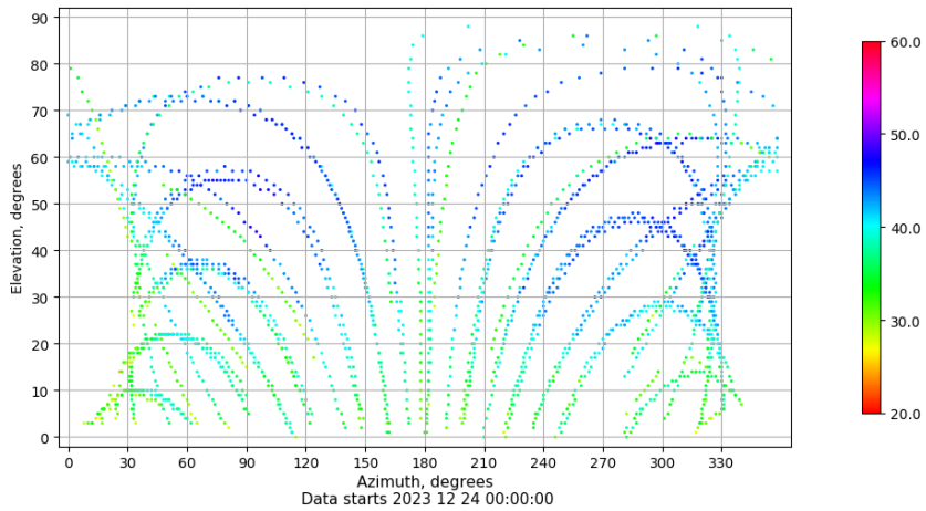
Azimuth-elevation plot for station ALC1. Signal to Noise S1C Data file ALC100ESP_R_2023358.xtr
