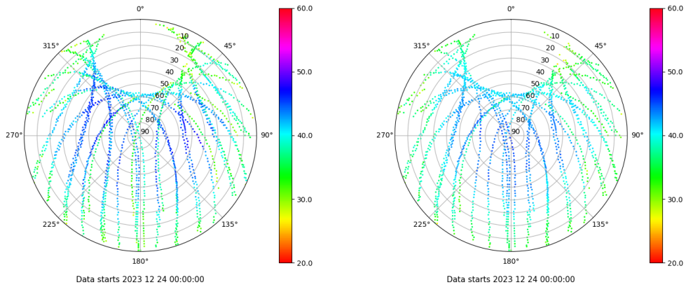
Skyplot for station ALC1. Signal to Noise S1C Data file ALC100ESP_R_2023358.xtr Skyplot for station ALC1. Signal to Noise S2C Data file ALC100ESP_R_2023358.xtr
