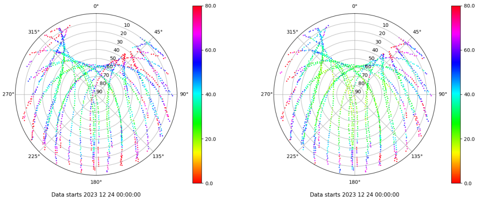
Skyplot for station ALC1. Parameter M1C Data file ALC100ESP_R_2023358.xtr Skyplot for station ALC1. Parameter M2C Data file ALC100ESP_R_2023358.xtr
