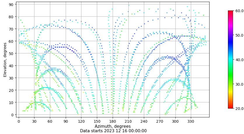
Azimuth-elevation plot for station ALC1. Signal to Noise S1C Data file ALC100ESP_R_2023350.xtr
