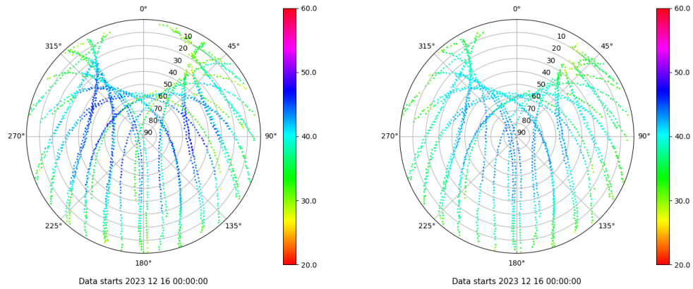
Skyplot for station ALC1. Signal to Noise S1C Data file ALC100ESP_R_2023350.xtr Skyplot for station ALC1. Signal to Noise S2C Data file ALC100ESP_R_2023350.xtr
