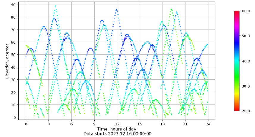
Time-elevation plot for station ALC1. Signal to Noise S1C Data file ALC100ESP_R_2023350.xtr
