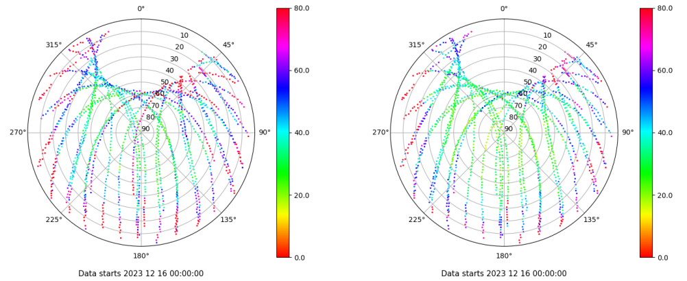
Skyplot for station ALC1. Parameter M1C Data file ALC100ESP_R_2023350.xtr Skyplot for station ALC1. Parameter M2C Data file ALC100ESP_R_2023350.xtr
