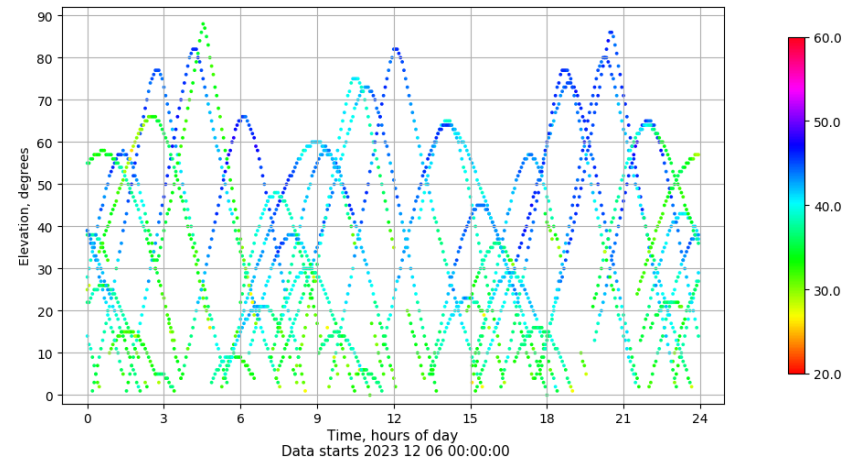
Time-elevation plot for station ALC1. Signal to Noise S1C Data file ALC100ESP_R_2023340.xtr
