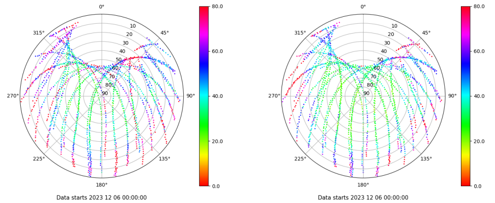
Skyplot for station ALC1. Parameter M1C Data file ALC100ESP_R_2023340.xtr Skyplot for station ALC1. Parameter M2C Data file ALC100ESP_R_2023340.xtr
