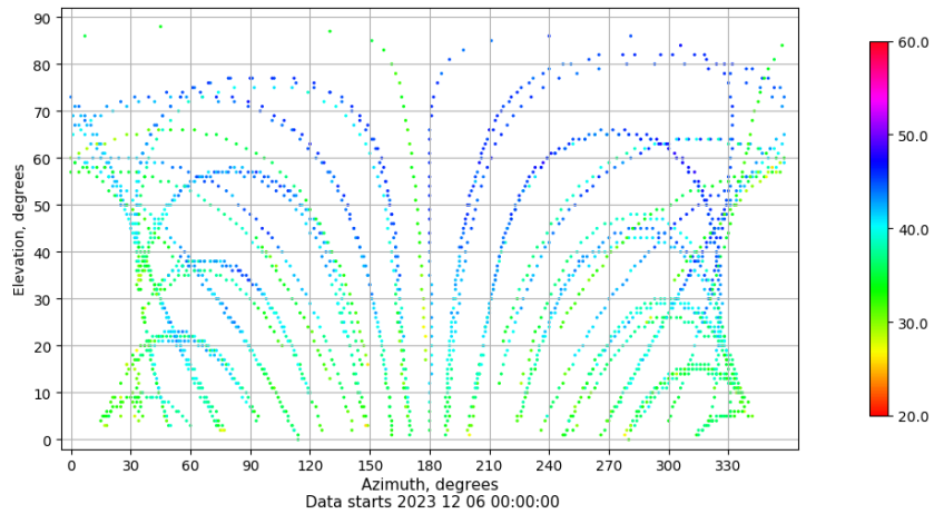
Azimuth-elevation plot for station ALC1. Signal to Noise S1C Data file ALC100ESP_R_2023340.xtr
