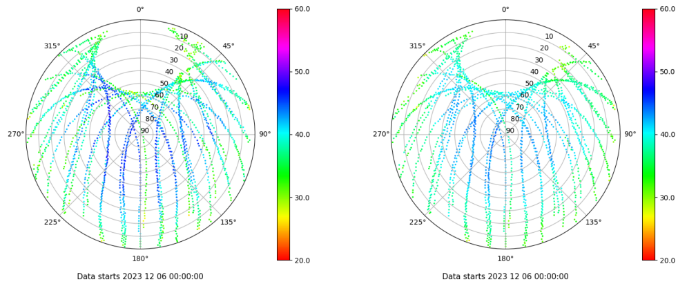
Skyplot for station ALC1. Signal to Noise S1C Data file ALC100ESP_R_2023340.xtr Skyplot for station ALC1. Signal to Noise S2C Data file ALC100ESP_R_2023340.xtr
