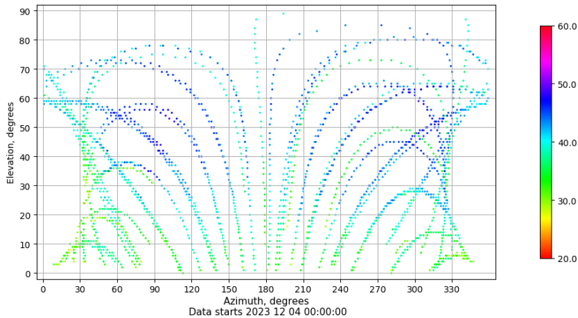
Azimuth-elevation plot for station ALC1. Signal to Noise S1C Data file ALC100ESP_R_2023338.xtr
