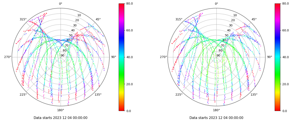
Skyplot for station ALC1. Parameter M1C Data file ALC100ESP_R_2023338.xtr Skyplot for station ALC1. Parameter M2C Data file ALC100ESP_R_2023338.xtr
