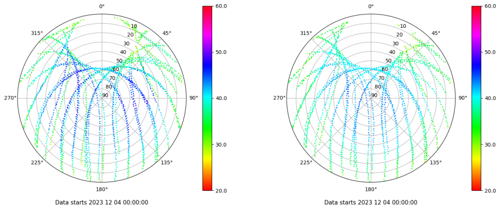
Skyplot for station ALC1. Signal to Noise S1C Data file ALC100ESP_R_2023338.xtr Skyplot for station ALC1. Signal to Noise S2C Data file ALC100ESP_R_2023338.xtr
