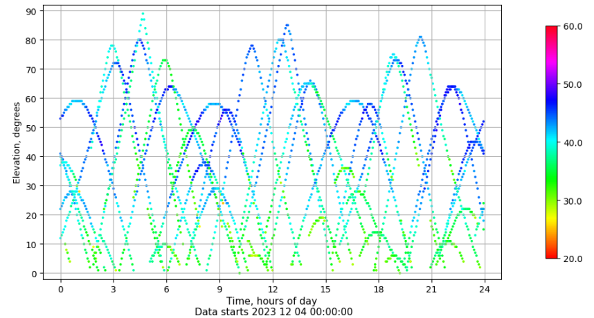
Time-elevation plot for station ALC1. Signal to Noise S1C Data file ALC100ESP_R_2023338.xtr
