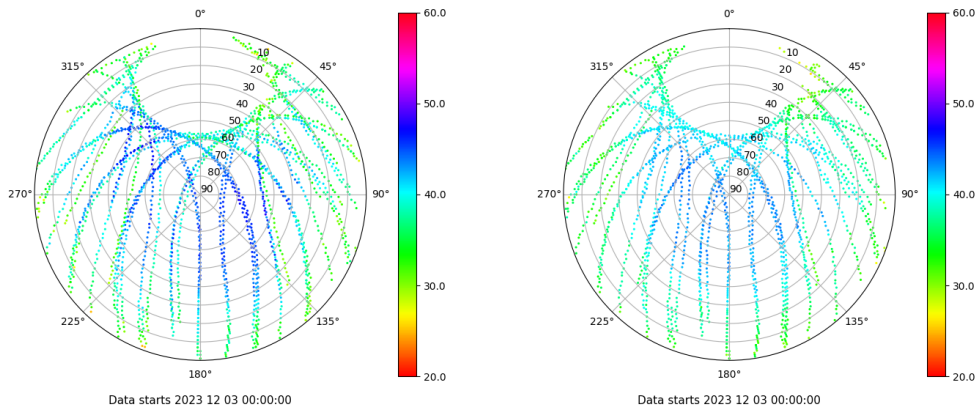
Skyplot for station ALC1. Signal to Noise S1C Data file ALC100ESP_R_2023337.xtr Skyplot for station ALC1. Signal to Noise S2C Data file ALC100ESP_R_2023337.xtr
