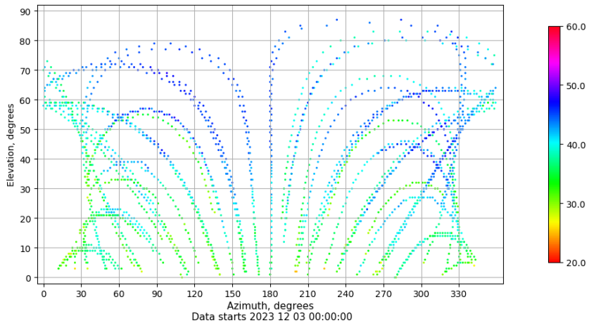
Azimuth-elevation plot for station ALC1. Signal to Noise S1C Data file ALC100ESP_R_2023337.xtr
