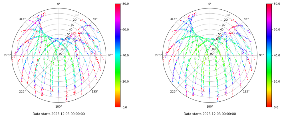
Skyplot for station ALC1. Parameter M1C Data file ALC100ESP_R_2023337.xtr Skyplot for station ALC1. Parameter M2C Data file ALC100ESP_R_2023337.xtr
