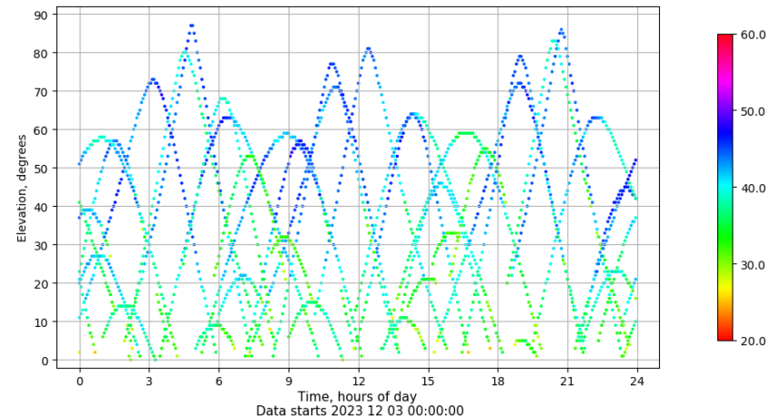
Time-elevation plot for station ALC1. Signal to Noise S1C Data file ALC100ESP_R_2023337.xtr
