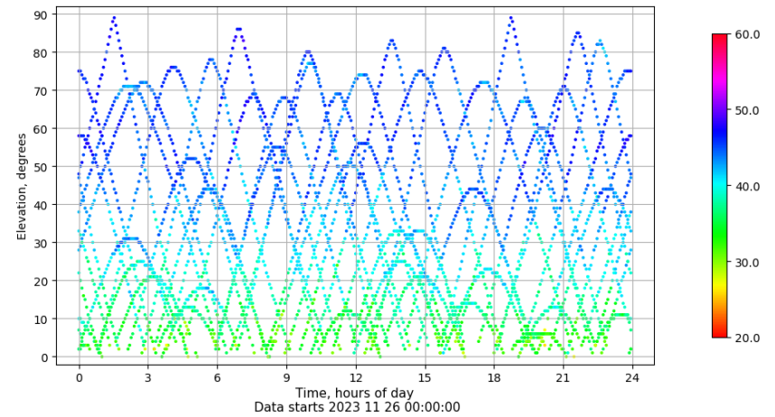
Time-elevation plot for station ALC1. Signal to Noise S1C Data file ALC100ESP_R_2023330.xtr
