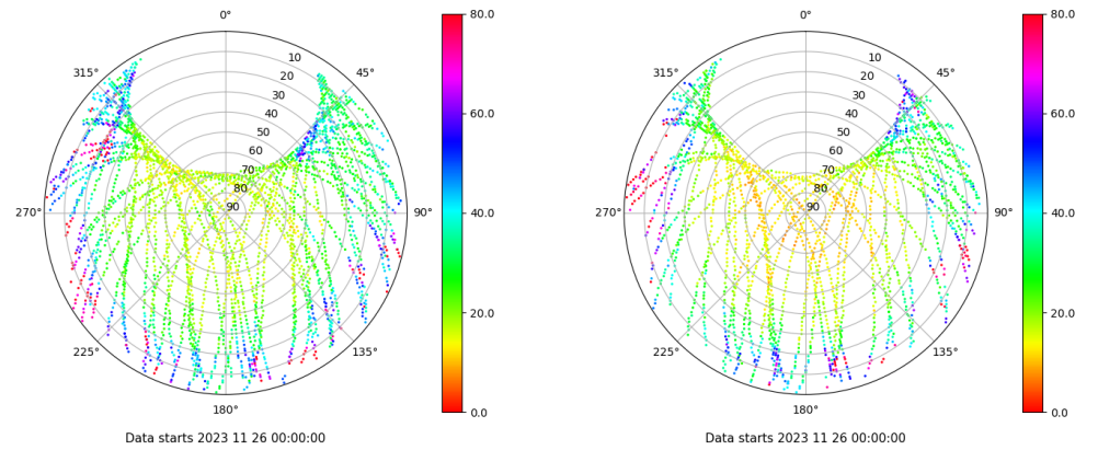
Skyplot for station ALC1. Parameter M1C Data file ALC100ESP_R_2023330.xtr Skyplot for station ALC1. Parameter M2X Data file ALC100ESP_R_2023330.xtr
