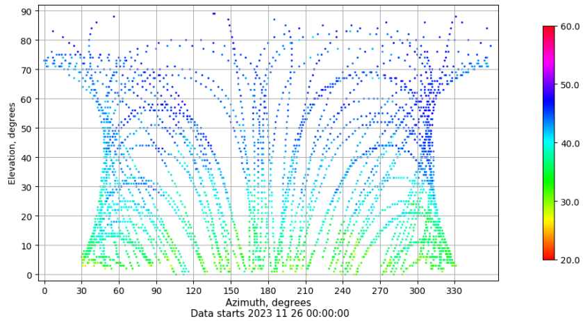
Azimuth-elevation plot for station ALC1. Signal to Noise S1C Data file ALC100ESP_R_2023330.xtr
