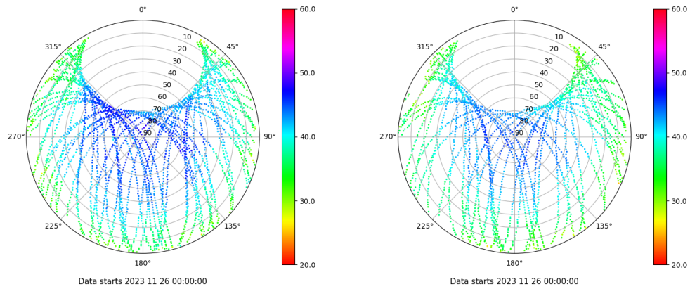
Skyplot for station ALC1. Signal to Noise S1C Data file ALC100ESP_R_2023330.xtr Skyplot for station ALC1. Signal to Noise S2X Data file ALC100ESP_R_2023330.xtr
