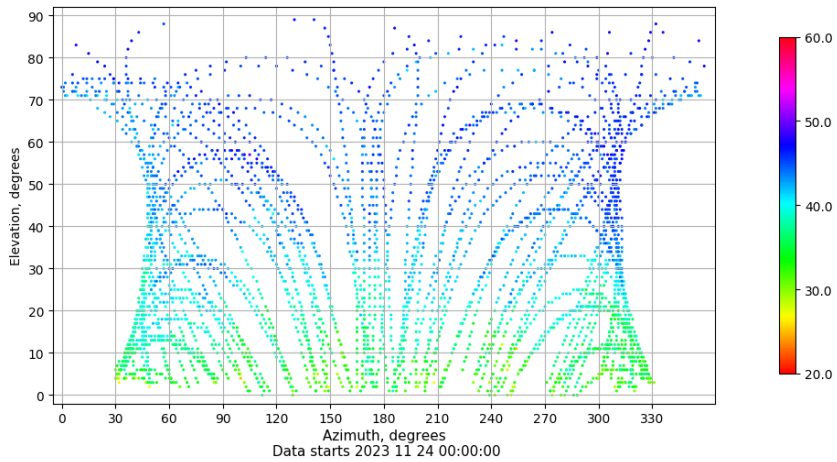
Azimuth-elevation plot for station ALC1. Signal to Noise S1C Data file ALC100ESP_R_2023328.xtr
