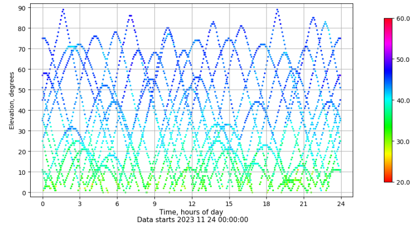
Time-elevation plot for station ALC1. Signal to Noise S1C Data file ALC100ESP_R_2023328.xtr
