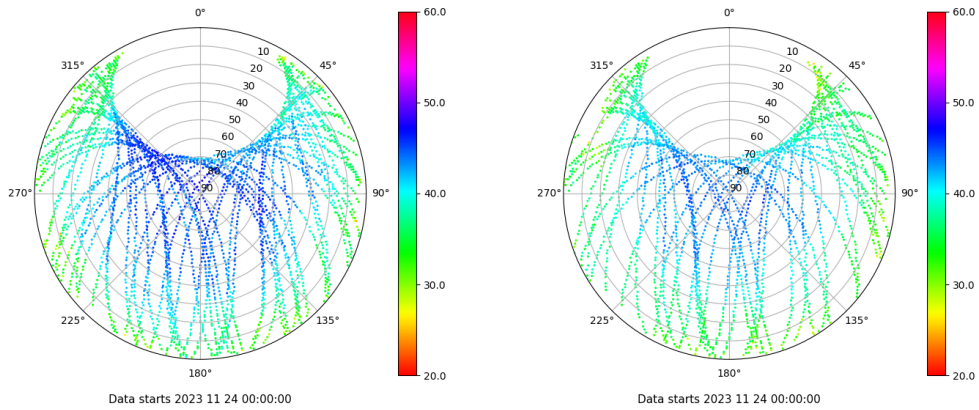
Skyplot for station ALC1. Signal to Noise S1C Data file ALC100ESP_R_2023328.xtr Skyplot for station ALC1. Signal to Noise S2X Data file ALC100ESP_R_2023328.xtr
