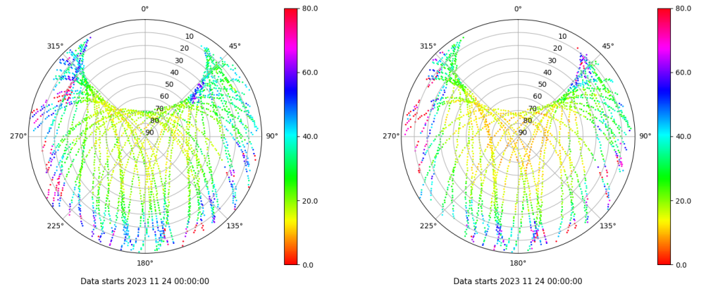
Skyplot for station ALC1. Parameter M1C Data file ALC100ESP_R_2023328.xtr Skyplot for station ALC1. Parameter M2X Data file ALC100ESP_R_2023328.xtr
