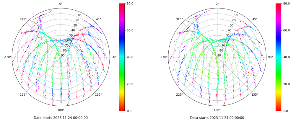
Skyplot for station ALC1. Parameter M1C Data file ALC100ESP_R_2023328.xtr Skyplot for station ALC1. Parameter M2C Data file ALC100ESP_R_2023328.xtr
