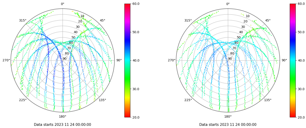
Skyplot for station ALC1. Signal to Noise S1C Data file ALC100ESP_R_2023328.xtr Skyplot for station ALC1. Signal to Noise S2C Data file ALC100ESP_R_2023328.xtr
