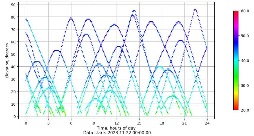
Time-elevation plot for station ALC1. Signal to Noise S1X Data file ALC100ESP_R_2023326.xtr
