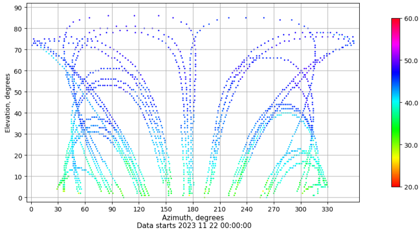
Azimuth-elevation plot for station ALC1. Signal to Noise S1X Data file ALC100ESP_R_2023326.xtr
