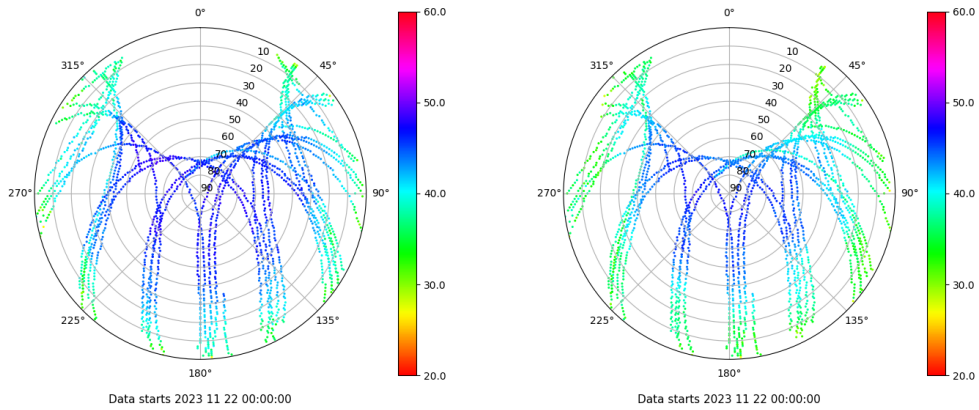
Skyplot for station ALC1. Signal to Noise S1X Data file ALC100ESP_R_2023326.xtr Skyplot for station ALC1. Signal to Noise S5X Data file ALC100ESP_R_2023326.xtr
