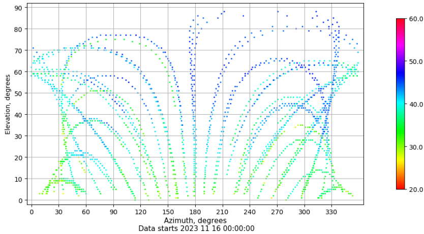
Azimuth-elevation plot for station ALC1. Signal to Noise S1C Data file ALC100ESP_R_2023320.xtr
