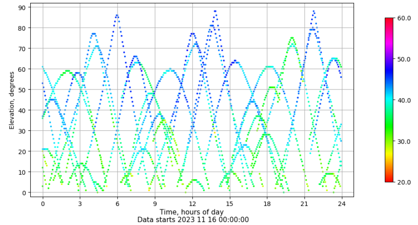
Time-elevation plot for station ALC1. Signal to Noise S1C Data file ALC100ESP_R_2023320.xtr
