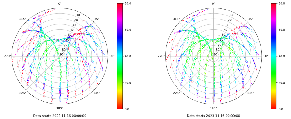
Skyplot for station ALC1. Parameter M1C Data file ALC100ESP_R_2023320.xtr Skyplot for station ALC1. Parameter M2C Data file ALC100ESP_R_2023320.xtr
