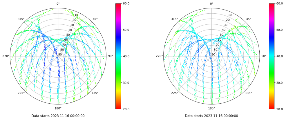
Skyplot for station ALC1. Signal to Noise S1C Data file ALC100ESP_R_2023320.xtr Skyplot for station ALC1. Signal to Noise S2C Data file ALC100ESP_R_2023320.xtr
