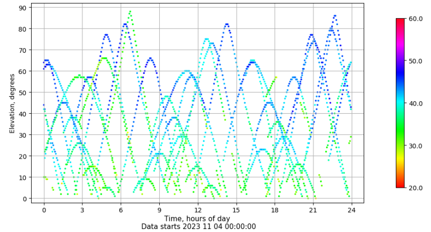
Time-elevation plot for station ALC1. Signal to Noise S1C Data file ALC100ESP_R_2023308.xtr
