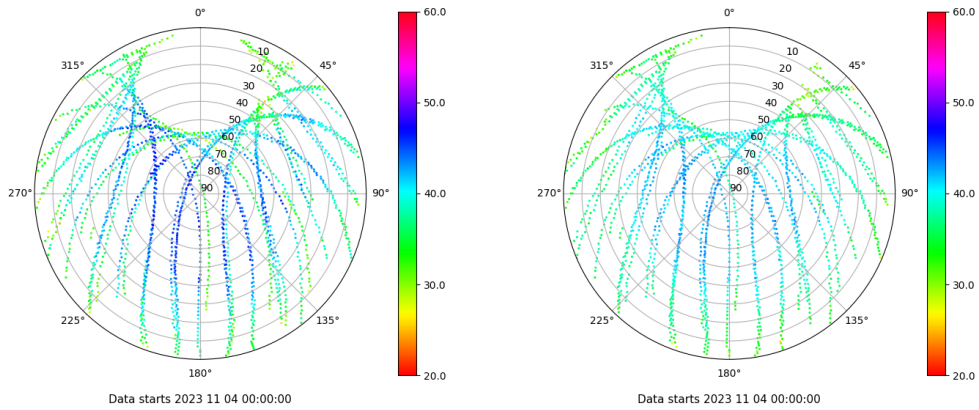
Skyplot for station ALC1. Signal to Noise S1C Data file ALC100ESP_R_2023308.xtr Skyplot for station ALC1. Signal to Noise S2C Data file ALC100ESP_R_2023308.xtr
