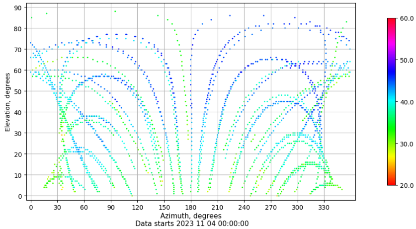
Azimuth-elevation plot for station ALC1. Signal to Noise S1C Data file ALC100ESP_R_2023308.xtr
