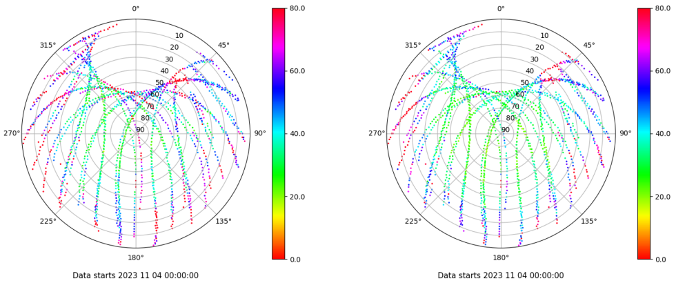
Skyplot for station ALC1. Parameter M1C Data file ALC100ESP_R_2023308.xtr Skyplot for station ALC1. Parameter M2C Data file ALC100ESP_R_2023308.xtr
