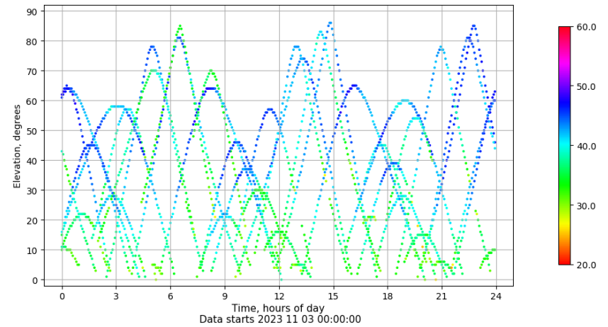
Time-elevation plot for station ALC1. Signal to Noise S1C Data file ALC100ESP_R_2023307.xtr
