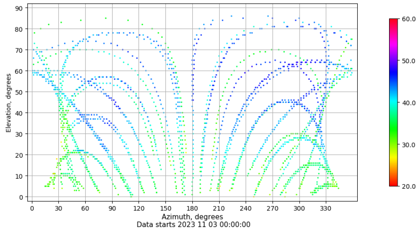
Azimuth-elevation plot for station ALC1. Signal to Noise S1C Data file ALC100ESP_R_2023307.xtr
