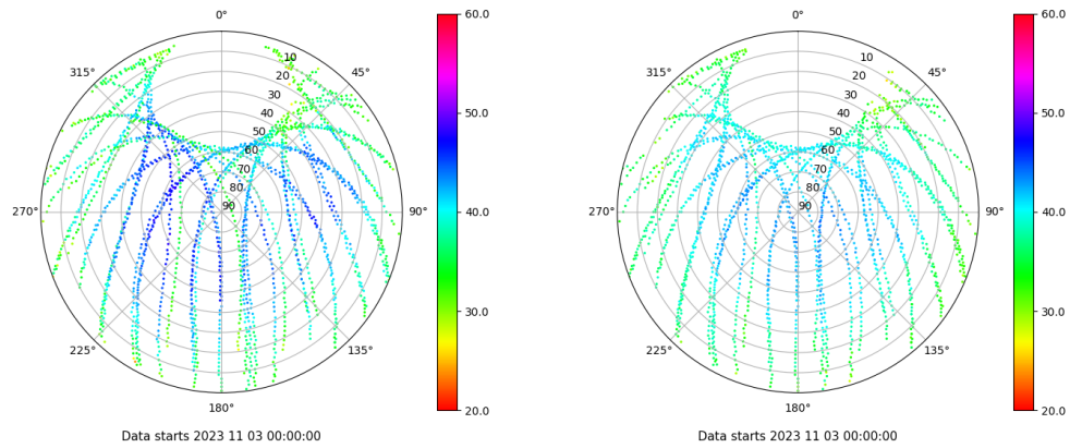
Skyplot for station ALC1. Signal to Noise S1C Data file ALC100ESP_R_2023307.xtr Skyplot for station ALC1. Signal to Noise S2C Data file ALC100ESP_R_2023307.xtr
