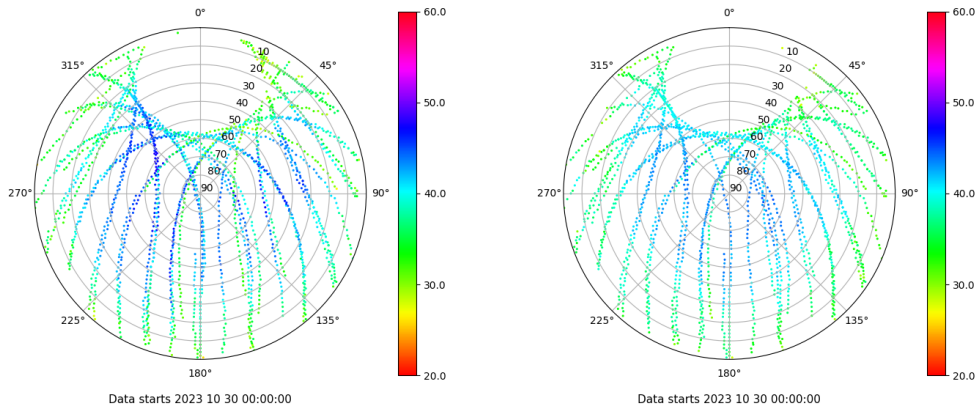
Skyplot for station ALC1. Signal to Noise S1C Data file ALC100ESP_R_2023303.xtr Skyplot for station ALC1. Signal to Noise S2C Data file ALC100ESP_R_2023303.xtr
