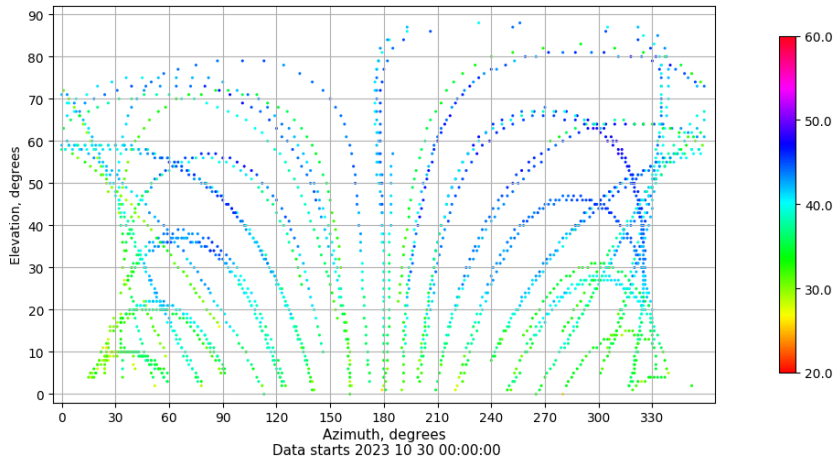
Azimuth-elevation plot for station ALC1. Signal to Noise S1C Data file ALC100ESP_R_2023303.xtr
