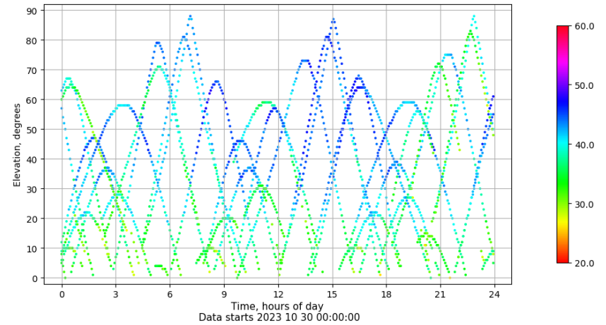
Time-elevation plot for station ALC1. Signal to Noise S1C Data file ALC100ESP_R_2023303.xtr
