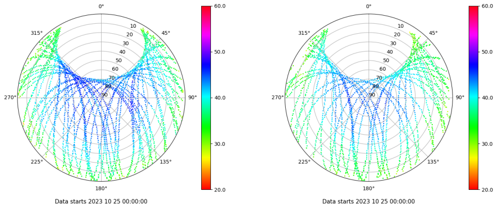
Skyplot for station ALC1. Signal to Noise S1C Data file ALC100ESP_R_2023298.xtr Skyplot for station ALC1. Signal to Noise S2X Data file ALC100ESP_R_2023298.xtr
