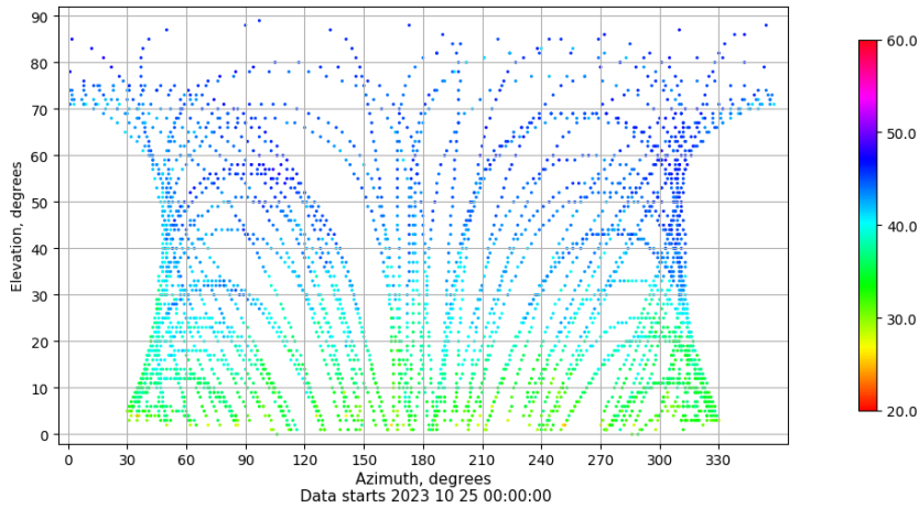
Azimuth-elevation plot for station ALC1. Signal to Noise S1C Data file ALC100ESP_R_2023298.xtr
