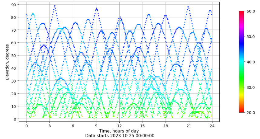
Time-elevation plot for station ALC1. Signal to Noise S1C Data file ALC100ESP_R_2023298.xtr
