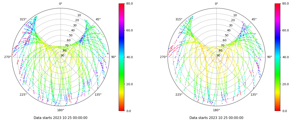
Skyplot for station ALC1. Parameter M1C Data file ALC100ESP_R_2023298.xtr Skyplot for station ALC1. Parameter M2X Data file ALC100ESP_R_2023298.xtr
