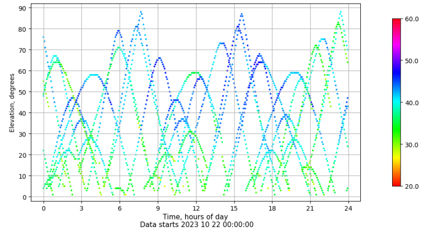
Time-elevation plot for station ALC1. Signal to Noise S1C Data file ALC100ESP_R_2023295.xtr
