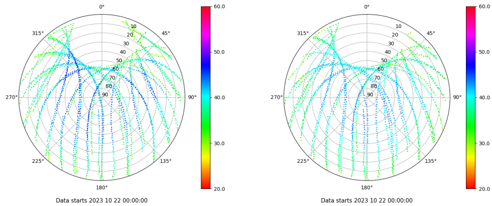
Skyplot for station ALC1. Signal to Noise S1C Data file ALC100ESP_R_2023295.xtr Skyplot for station ALC1. Signal to Noise S2C Data file ALC100ESP_R_2023295.xtr
