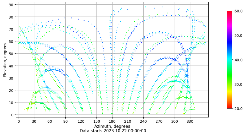
Azimuth-elevation plot for station ALC1. Signal to Noise S1C Data file ALC100ESP_R_2023295.xtr
