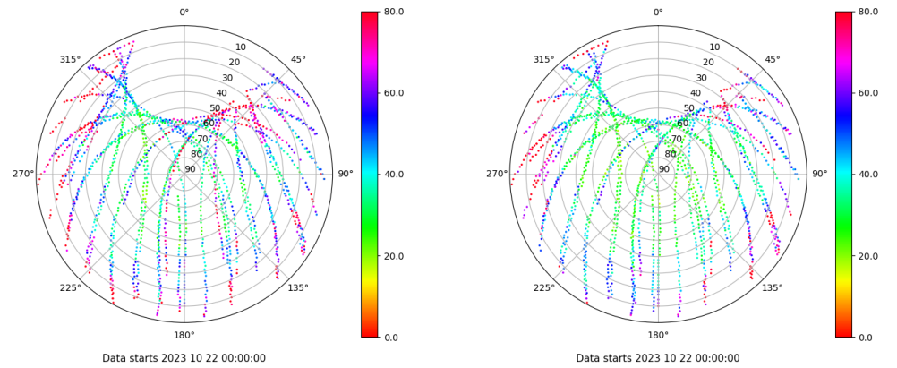
Skyplot for station ALC1. Parameter M1C Data file ALC100ESP_R_2023295.xtr Skyplot for station ALC1. Parameter M2C Data file ALC100ESP_R_2023295.xtr
