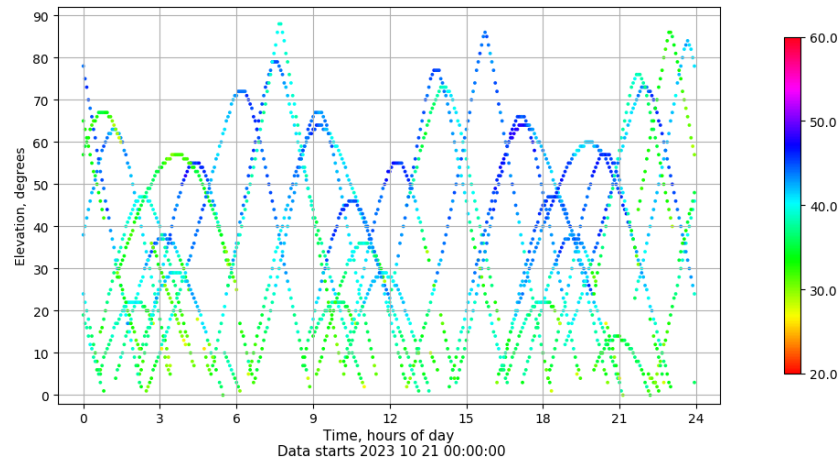
Time-elevation plot for station ALC1. Signal to Noise S1C Data file ALC100ESP_R_2023294.xtr
