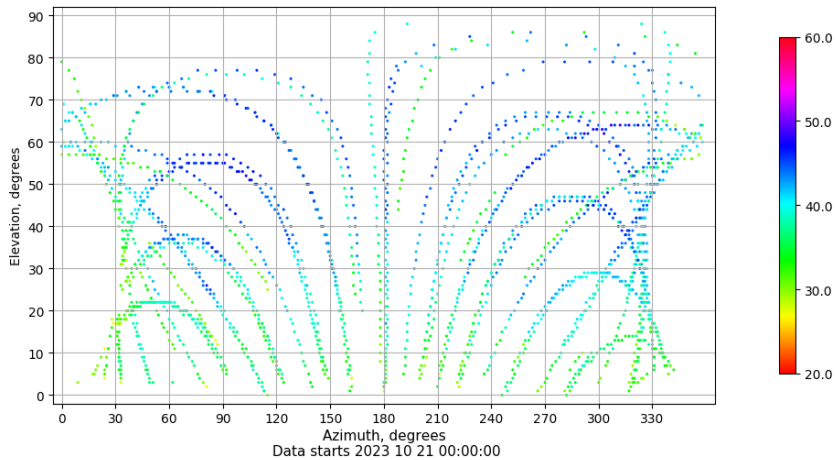
Azimuth-elevation plot for station ALC1. Signal to Noise S1C Data file ALC100ESP_R_2023294.xtr
