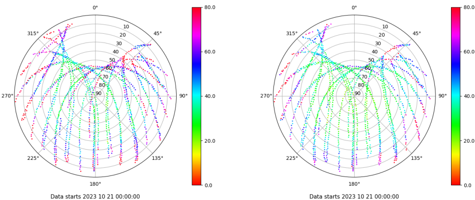
Skyplot for station ALC1. Parameter M1C Data file ALC100ESP_R_2023294.xtr Skyplot for station ALC1. Parameter M2C Data file ALC100ESP_R_2023294.xtr
