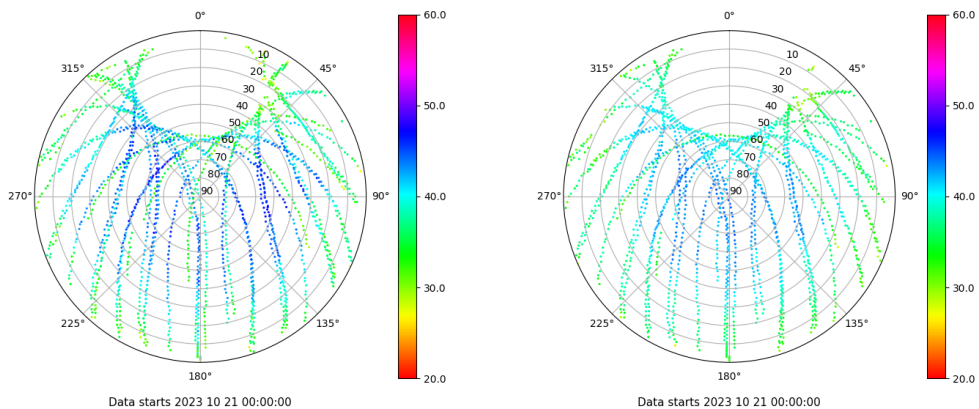
Skyplot for station ALC1. Signal to Noise S1C Data file ALC100ESP_R_2023294.xtr Skyplot for station ALC1. Signal to Noise S2C Data file ALC100ESP_R_2023294.xtr
