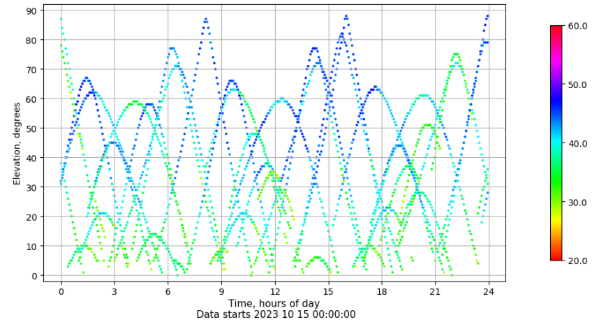
Time-elevation plot for station ALC1. Signal to Noise S1C Data file ALC100ESP_R_2023288.xtr
