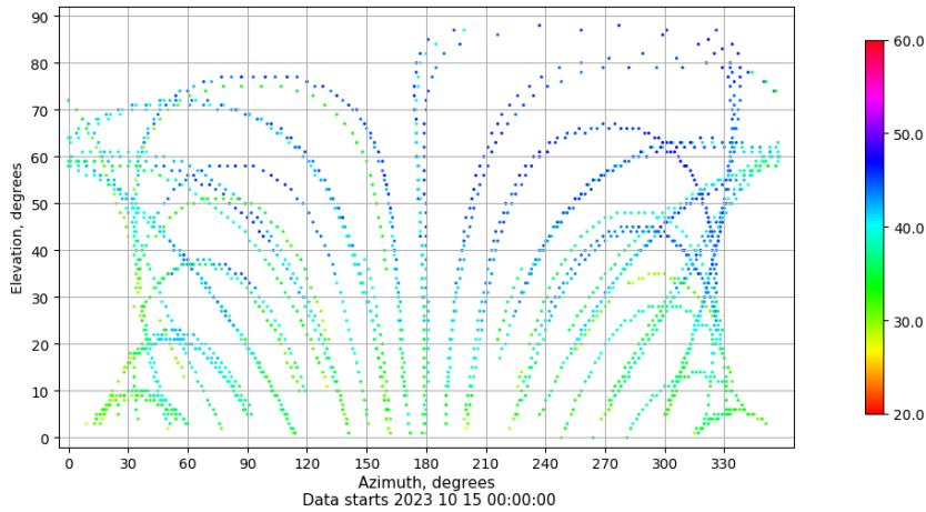
Azimuth-elevation plot for station ALC1. Signal to Noise S1C Data file ALC100ESP_R_2023288.xtr
