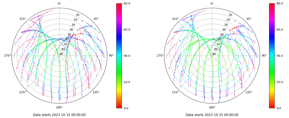
Skyplot for station ALC1. Parameter M1C Data file ALC100ESP_R_2023288.xtr Skyplot for station ALC1. Parameter M2C Data file ALC100ESP_R_2023288.xtr
