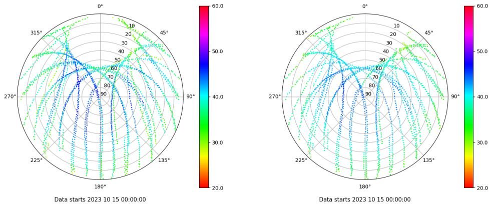
Skyplot for station ALC1. Signal to Noise S1C Data file ALC100ESP_R_2023288.xtr Skyplot for station ALC1. Signal to Noise S2C Data file ALC100ESP_R_2023288.xtr
