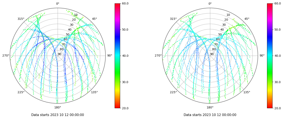
Skyplot for station ALC1. Signal to Noise S1C Data file ALC100ESP_R_2023285.xtr Skyplot for station ALC1. Signal to Noise S2C Data file ALC100ESP_R_2023285.xtr
