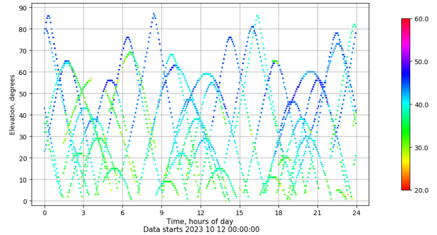
Time-elevation plot for station ALC1. Signal to Noise S1C Data file ALC100ESP_R_2023285.xtr
