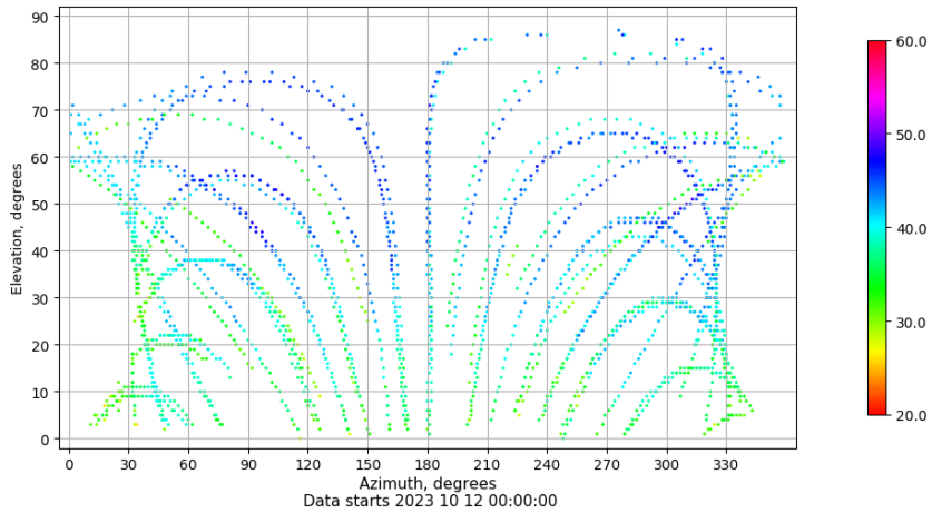
Azimuth-elevation plot for station ALC1. Signal to Noise S1C Data file ALC100ESP_R_2023285.xtr
