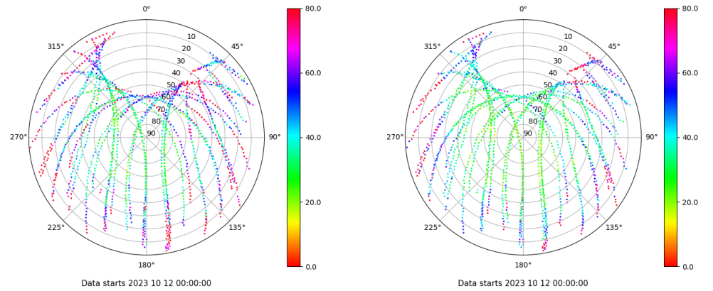
Skyplot for station ALC1. Parameter M1C Data file ALC100ESP_R_2023285.xtr Skyplot for station ALC1. Parameter M2C Data file ALC100ESP_R_2023285.xtr
