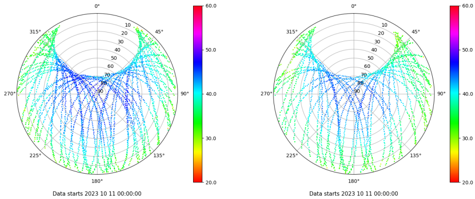
Skyplot for station ALC1. Signal to Noise S1C Data file ALC100ESP_R_2023284.xtr Skyplot for station ALC1. Signal to Noise S2X Data file ALC100ESP_R_2023284.xtr
