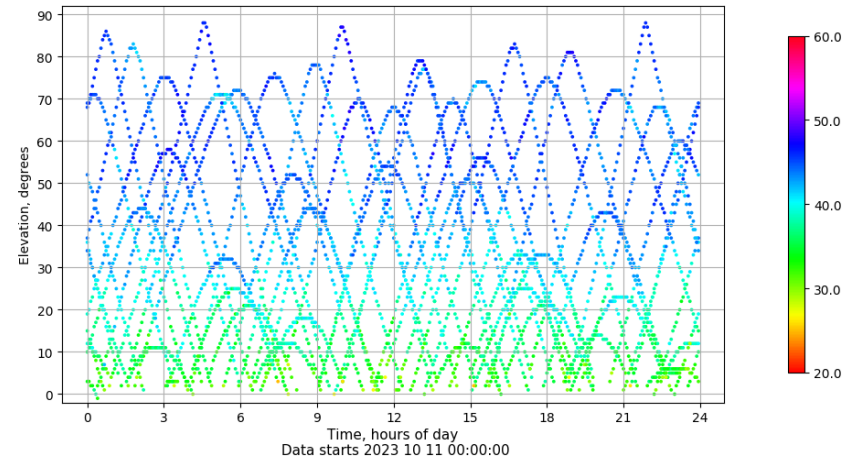
Time-elevation plot for station ALC1. Signal to Noise S1C Data file ALC100ESP_R_2023284.xtr
