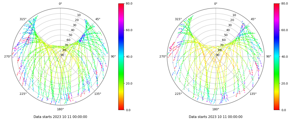
Skyplot for station ALC1. Parameter M1C Data file ALC100ESP_R_2023284.xtr Skyplot for station ALC1. Parameter M2X Data file ALC100ESP_R_2023284.xtr
