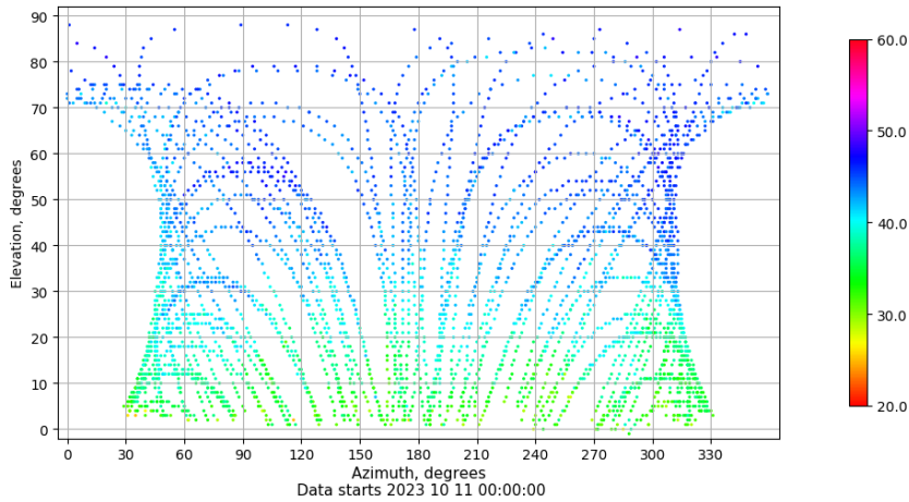
Azimuth-elevation plot for station ALC1. Signal to Noise S1C Data file ALC100ESP_R_2023284.xtr
