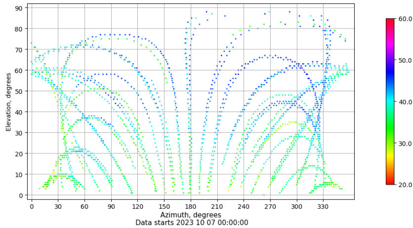
Azimuth-elevation plot for station ALC1. Signal to Noise S1C Data file ALC100ESP_R_2023280.xtr
