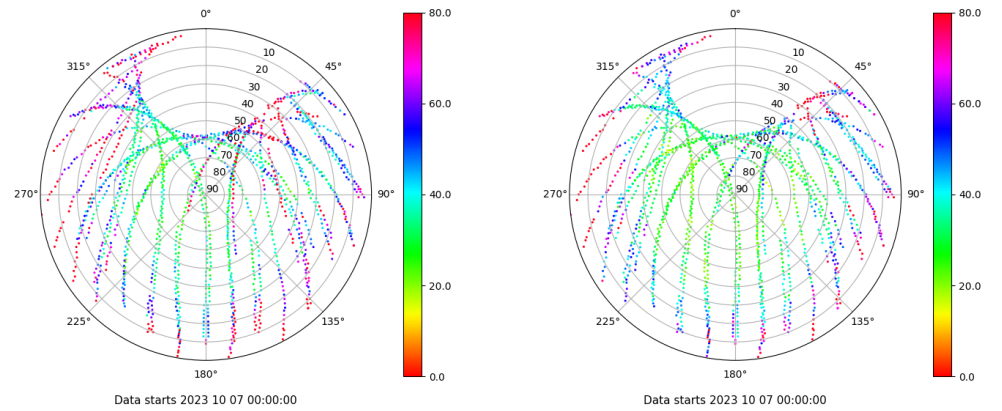
Skyplot for station ALC1. Parameter M1C Data file ALC100ESP_R_2023280.xtr Skyplot for station ALC1. Parameter M2C Data file ALC100ESP_R_2023280.xtr
