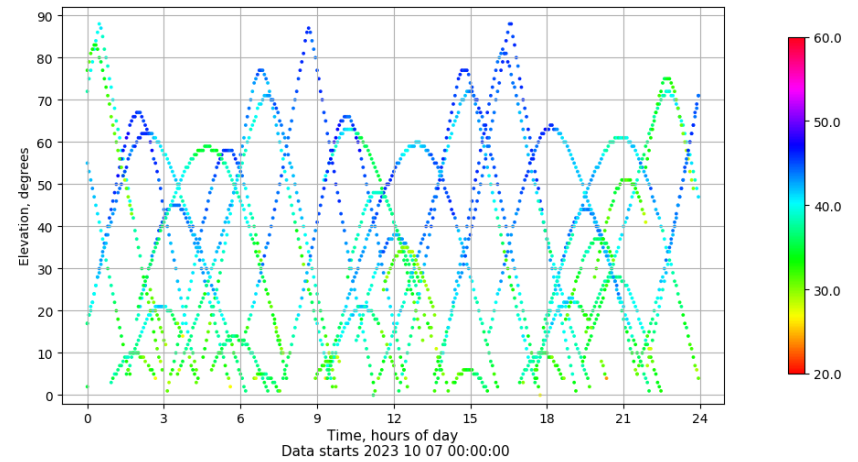
Time-elevation plot for station ALC1. Signal to Noise S1C Data file ALC100ESP_R_2023280.xtr
