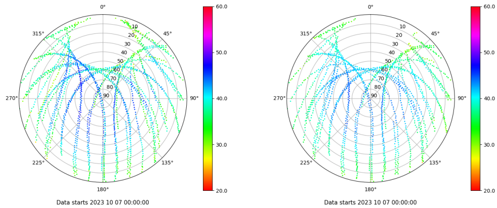
Skyplot for station ALC1. Signal to Noise S1C Data file ALC100ESP_R_2023280.xtr Skyplot for station ALC1. Signal to Noise S2C Data file ALC100ESP_R_2023280.xtr
