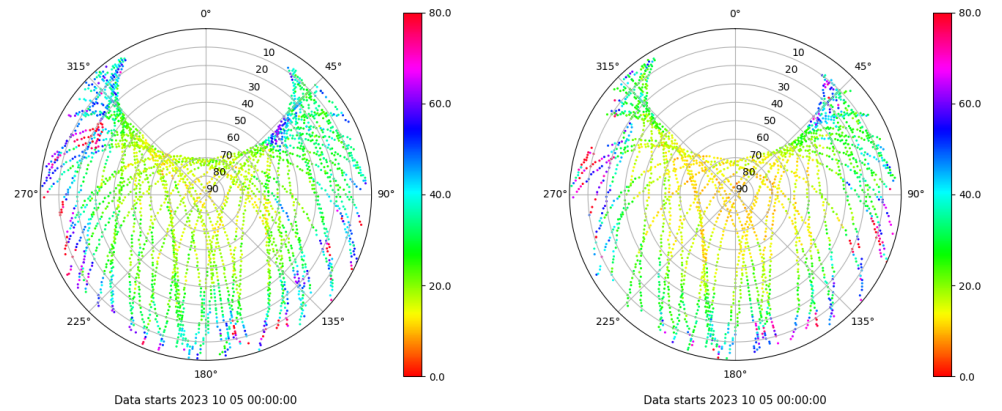
Skyplot for station ALC1. Parameter M1C Data file ALC100ESP_R_2023278.xtr Skyplot for station ALC1. Parameter M2X Data file ALC100ESP_R_2023278.xtr
