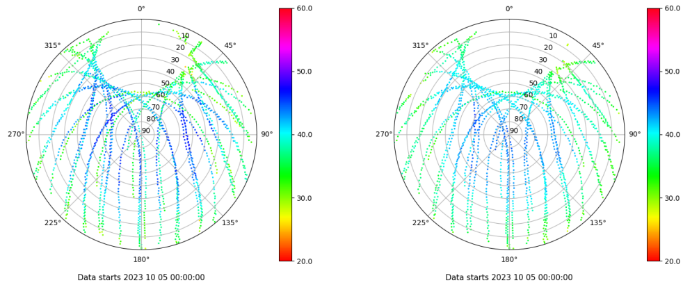
Skyplot for station ALC1. Signal to Noise S1C Data file ALC100ESP_R_2023278.xtr Skyplot for station ALC1. Signal to Noise S2C Data file ALC100ESP_R_2023278.xtr
