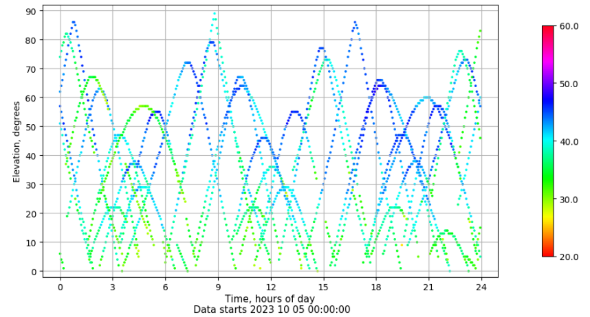
Time-elevation plot for station ALC1. Signal to Noise S1C Data file ALC100ESP_R_2023278.xtr
