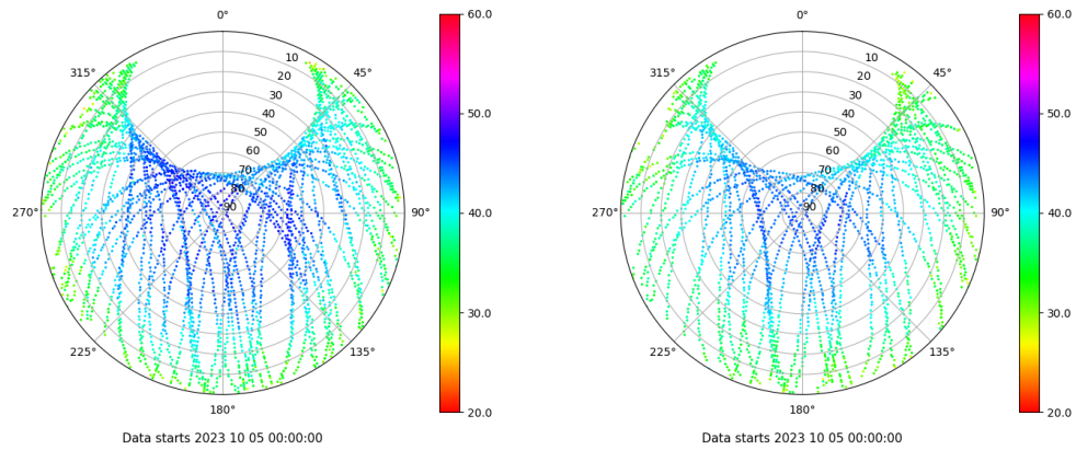
Skyplot for station ALC1. Signal to Noise S1C Data file ALC100ESP_R_2023278.xtr Skyplot for station ALC1. Signal to Noise S2X Data file ALC100ESP_R_2023278.xtr
