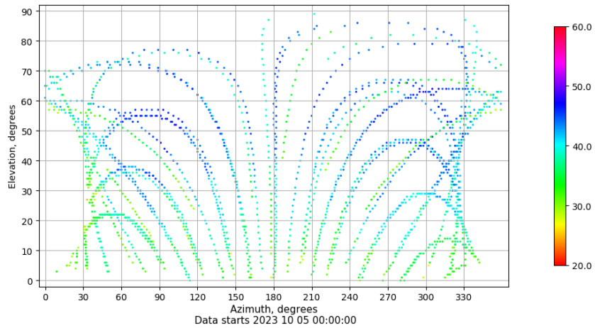
Azimuth-elevation plot for station ALC1. Signal to Noise S1C Data file ALC100ESP_R_2023278.xtr
