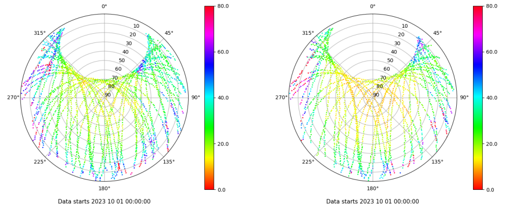
Skyplot for station ALC1. Parameter M1C Data file ALC100ESP_R_2023274.xtr Skyplot for station ALC1. Parameter M2X Data file ALC100ESP_R_2023274.xtr
