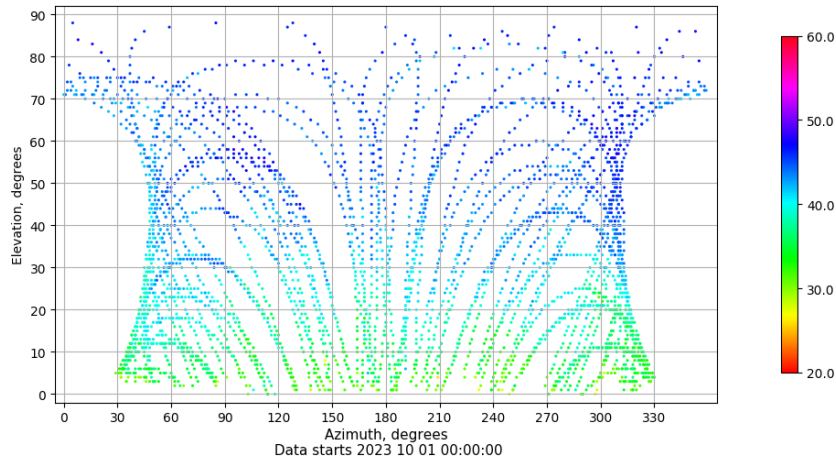
Azimuth-elevation plot for station ALC1. Signal to Noise S1C Data file ALC100ESP_R_2023274.xtr
