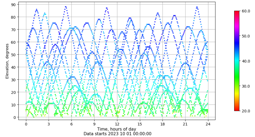
Time-elevation plot for station ALC1. Signal to Noise S1C Data file ALC100ESP_R_2023274.xtr
