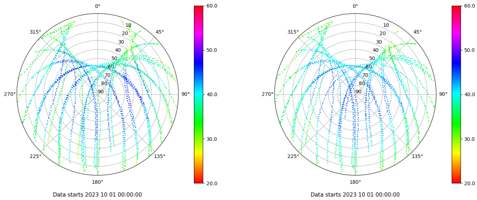
Skyplot for station ALC1. Signal to Noise S1C Data file ALC100ESP_R_2023274.xtr Skyplot for station ALC1. Signal to Noise S2C Data file ALC100ESP_R_2023274.xtr
