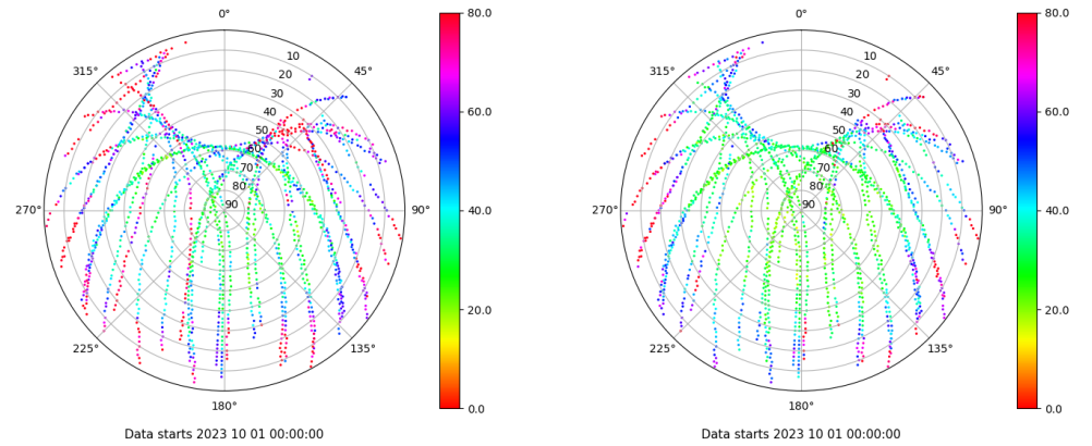
Skyplot for station ALC1. Parameter M1C Data file ALC100ESP_R_2023274.xtr Skyplot for station ALC1. Parameter M2C Data file ALC100ESP_R_2023274.xtr
