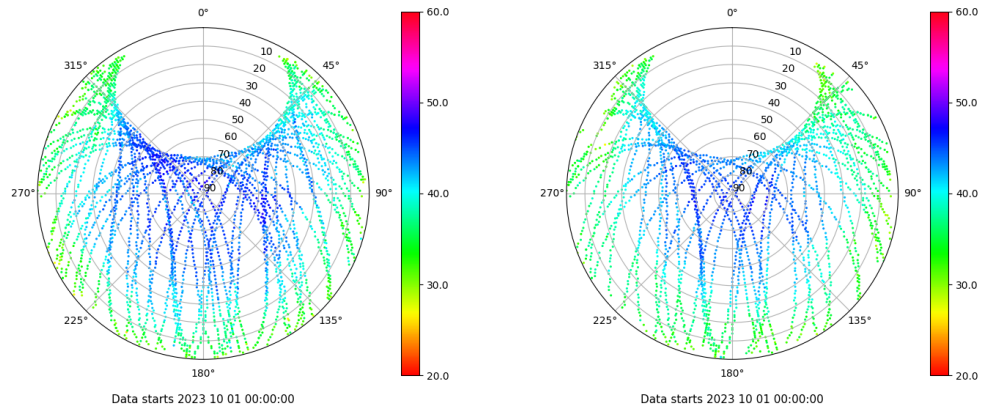
Skyplot for station ALC1. Signal to Noise S1C Data file ALC100ESP_R_2023274.xtr Skyplot for station ALC1. Signal to Noise S2X Data file ALC100ESP_R_2023274.xtr
