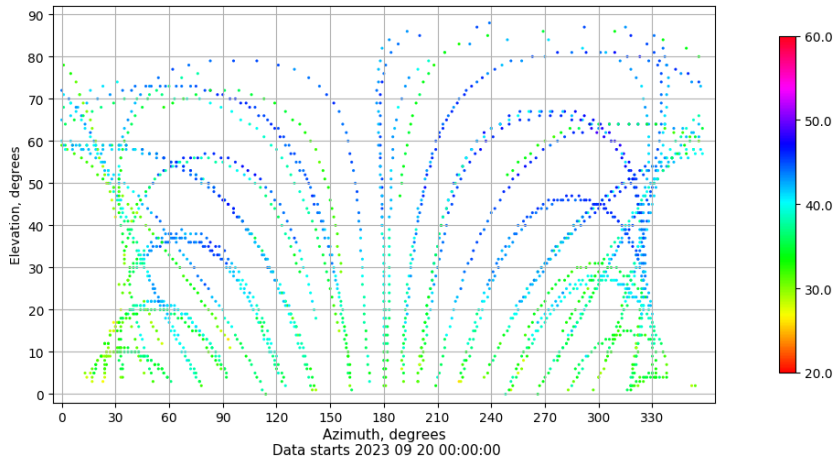
Azimuth-elevation plot for station ALC1. Signal to Noise S1C Data file ALC100ESP_R_2023263.xtr
