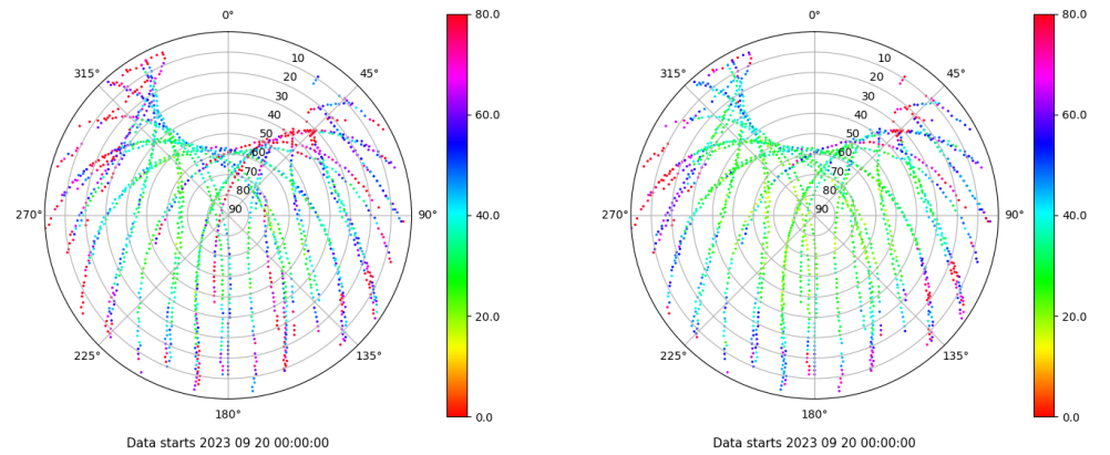
Skyplot for station ALC1. Parameter M1C Data file ALC100ESP_R_2023263.xtr Skyplot for station ALC1. Parameter M2C Data file ALC100ESP_R_2023263.xtr
