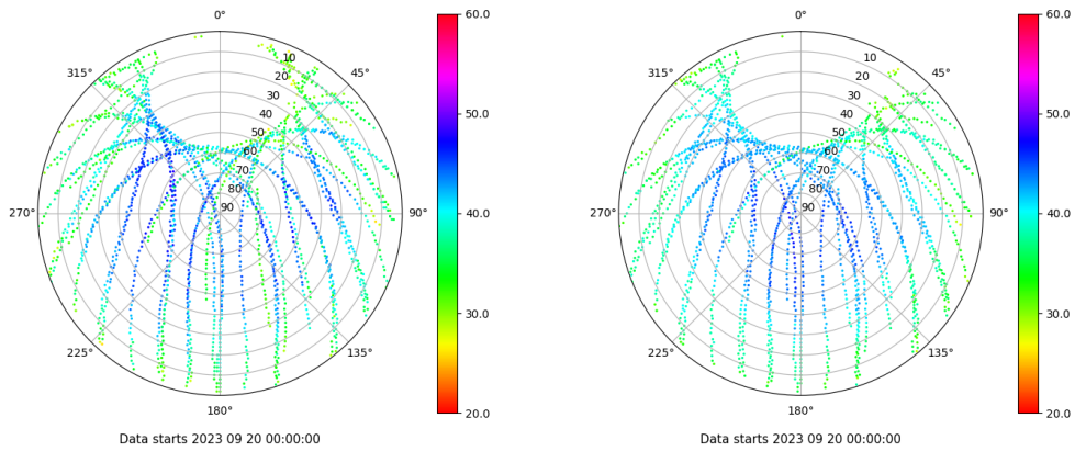
Skyplot for station ALC1. Signal to Noise S1C Data file ALC100ESP_R_2023263.xtr Skyplot for station ALC1. Signal to Noise S2C Data file ALC100ESP_R_2023263.xtr
