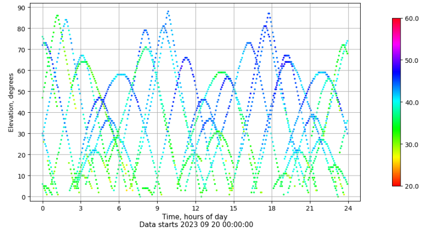
Time-elevation plot for station ALC1. Signal to Noise S1C Data file ALC100ESP_R_2023263.xtr
