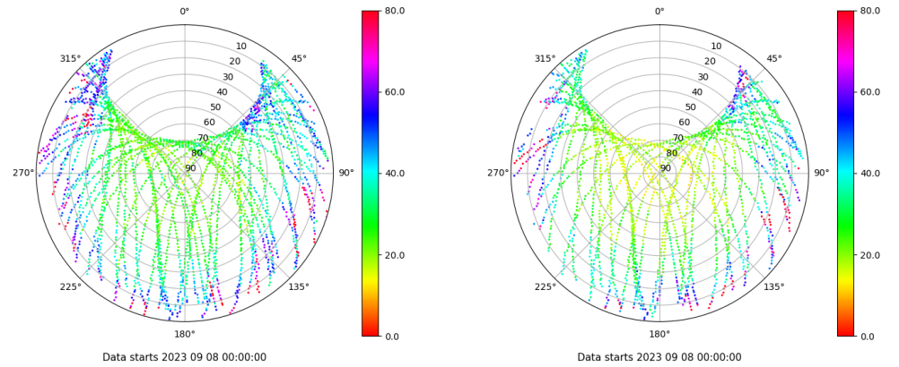
Skyplot for station ALC1. Parameter M1C Data file ALC100ESP_R_2023251.xtr Skyplot for station ALC1. Parameter M2X Data file ALC100ESP_R_2023251.xtr
