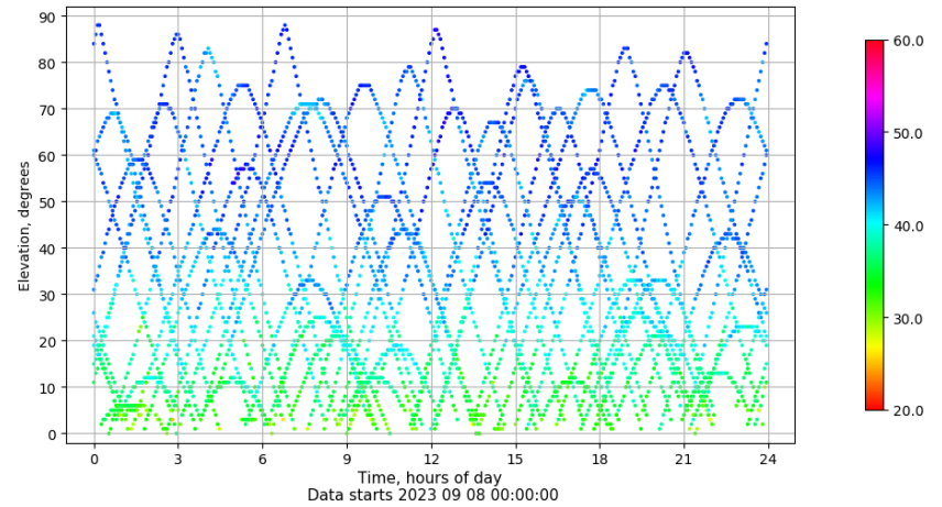
Time-elevation plot for station ALC1. Signal to Noise S1C Data file ALC100ESP_R_2023251.xtr
