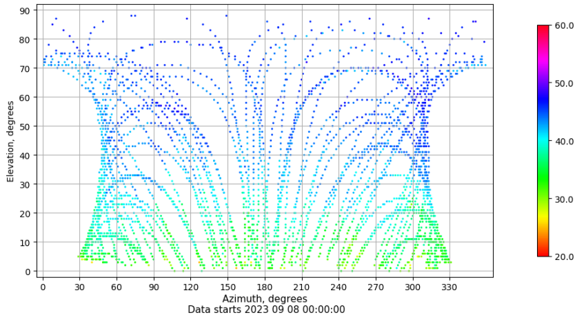
Azimuth-elevation plot for station ALC1. Signal to Noise S1C Data file ALC100ESP_R_2023251.xtr
