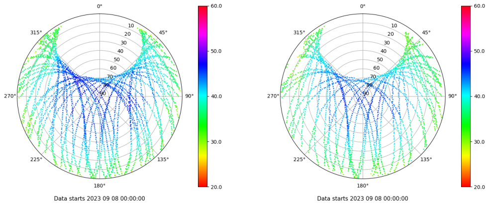
Skyplot for station ALC1. Signal to Noise S1C Data file ALC100ESP_R_2023251.xtr Skyplot for station ALC1. Signal to Noise S2X Data file ALC100ESP_R_2023251.xtr
