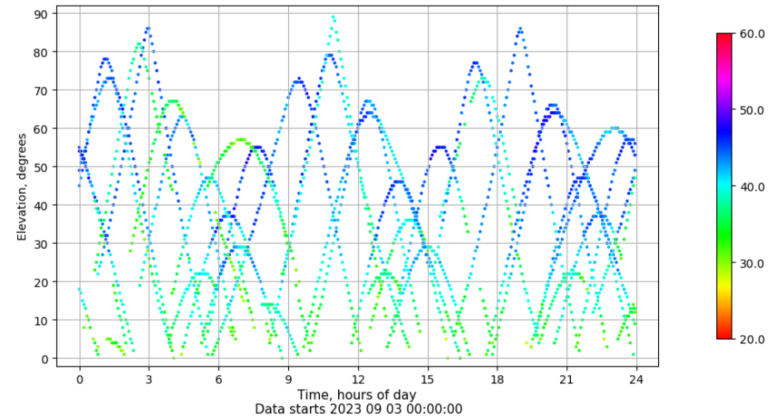
Time-elevation plot for station ALC1. Signal to Noise S1C Data file ALC100ESP_R_2023246.xtr
