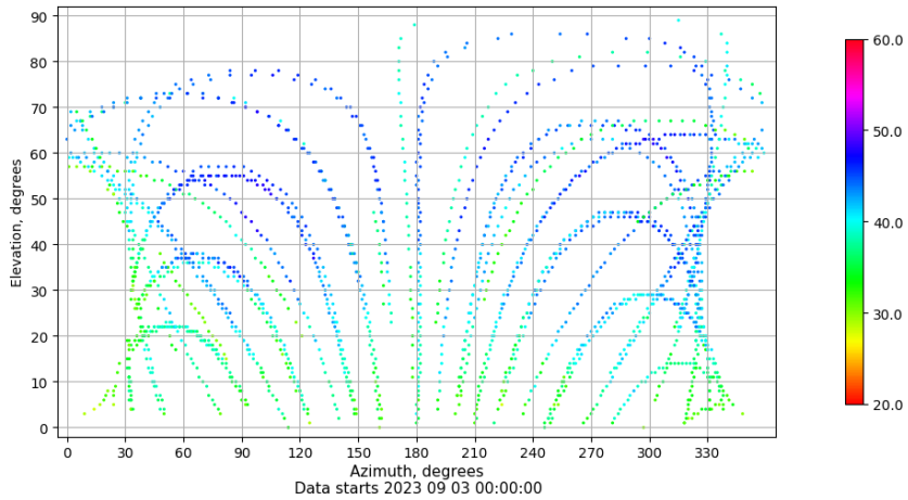
Azimuth-elevation plot for station ALC1. Signal to Noise S1C Data file ALC100ESP_R_2023246.xtr
