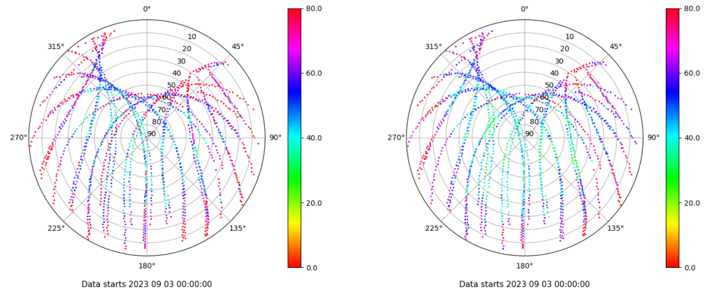
Skyplot for station ALC1. Parameter M1C Data file ALC100ESP_R_2023246.xtr Skyplot for station ALC1. Parameter M2C Data file ALC100ESP_R_2023246.xtr
