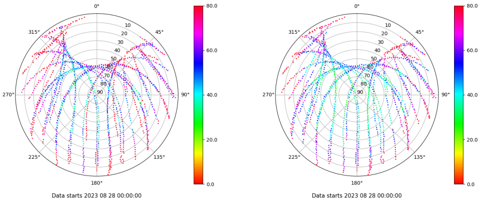
Skyplot for station ALC1. Parameter M1C Data file ALC100ESP_R_2023240.xtr Skyplot for station ALC1. Parameter M2C Data file ALC100ESP_R_2023240.xtr
