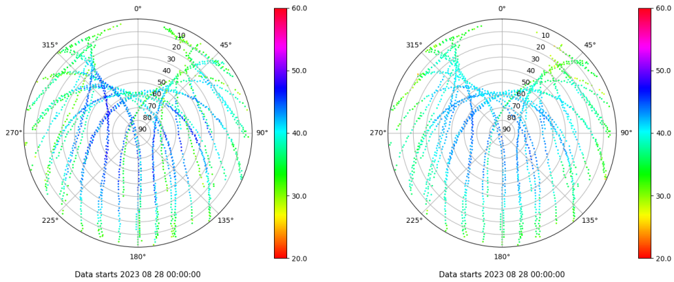
Skyplot for station ALC1. Signal to Noise S1C Data file ALC100ESP_R_2023240.xtr Skyplot for station ALC1. Signal to Noise S2C Data file ALC100ESP_R_2023240.xtr
