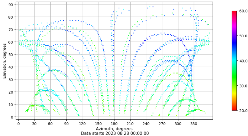
Azimuth-elevation plot for station ALC1. Signal to Noise S1C Data file ALC100ESP_R_2023240.xtr
