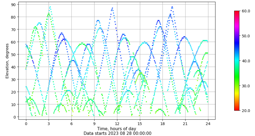
Time-elevation plot for station ALC1. Signal to Noise S1C Data file ALC100ESP_R_2023240.xtr
