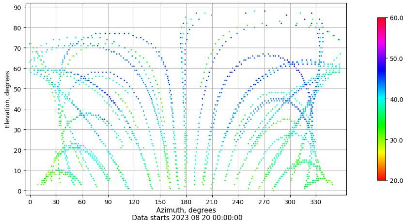
Azimuth-elevation plot for station ALC1. Signal to Noise S1C Data file ALC100ESP_R_2023232.xtr
