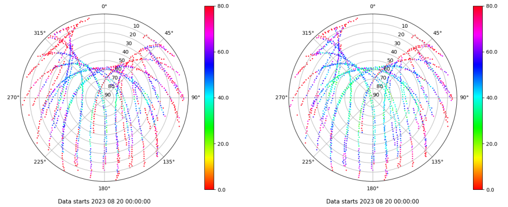
Skyplot for station ALC1. Parameter M1C Data file ALC100ESP_R_2023232.xtr Skyplot for station ALC1. Parameter M2C Data file ALC100ESP_R_2023232.xtr
