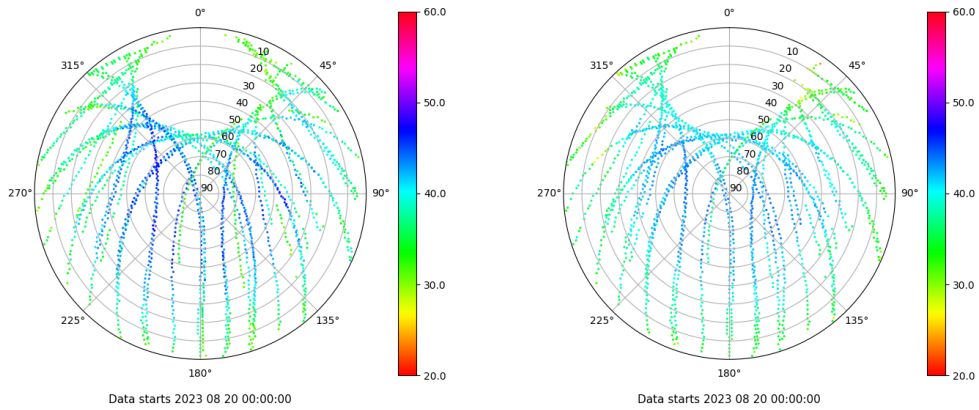
Skyplot for station ALC1. Signal to Noise S1C Data file ALC100ESP_R_2023232.xtr Skyplot for station ALC1. Signal to Noise S2C Data file ALC100ESP_R_2023232.xtr
