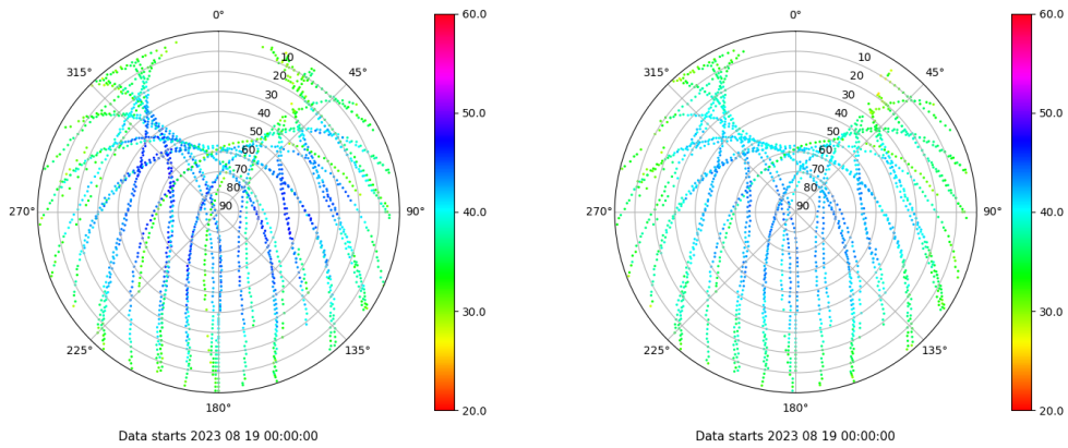
Skyplot for station ALC1. Signal to Noise S1C Data file ALC100ESP_R_2023231.xtr Skyplot for station ALC1. Signal to Noise S2C Data file ALC100ESP_R_2023231.xtr
