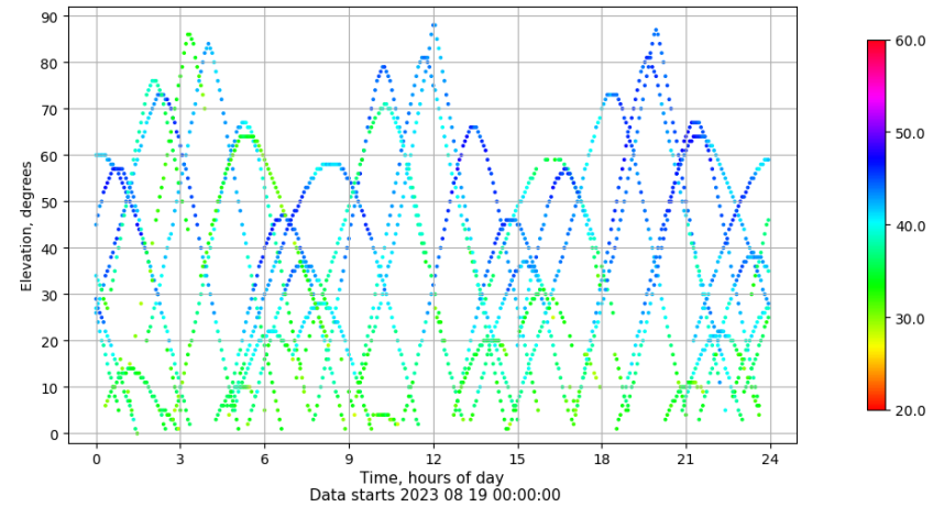
Time-elevation plot for station ALC1. Signal to Noise S1C Data file ALC100ESP_R_2023231.xtr
