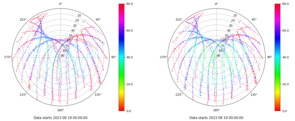
Skyplot for station ALC1. Parameter M1C Data file ALC100ESP_R_2023231.xtr Skyplot for station ALC1. Parameter M2C Data file ALC100ESP_R_2023231.xtr
