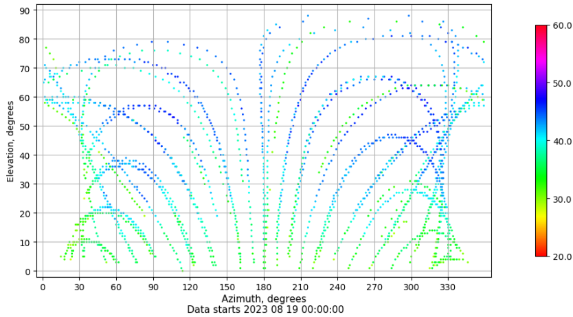
Azimuth-elevation plot for station ALC1. Signal to Noise S1C Data file ALC100ESP_R_2023231.xtr
