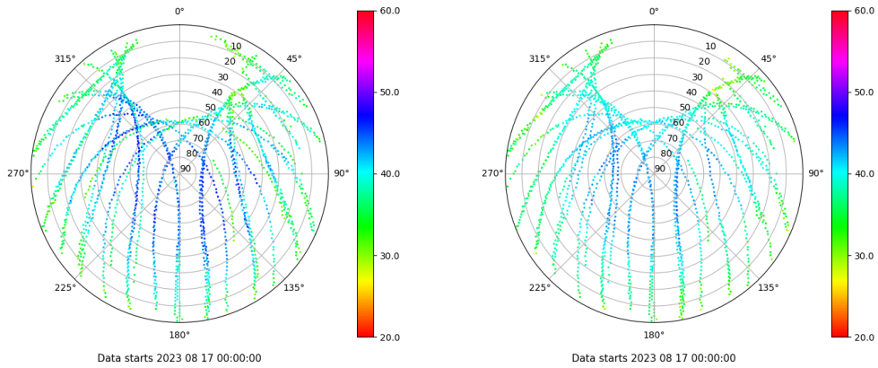
Skyplot for station ALC1. Signal to Noise S1C Data file ALC100ESP_R_2023229.xtr Skyplot for station ALC1. Signal to Noise S2C Data file ALC100ESP_R_2023229.xtr
