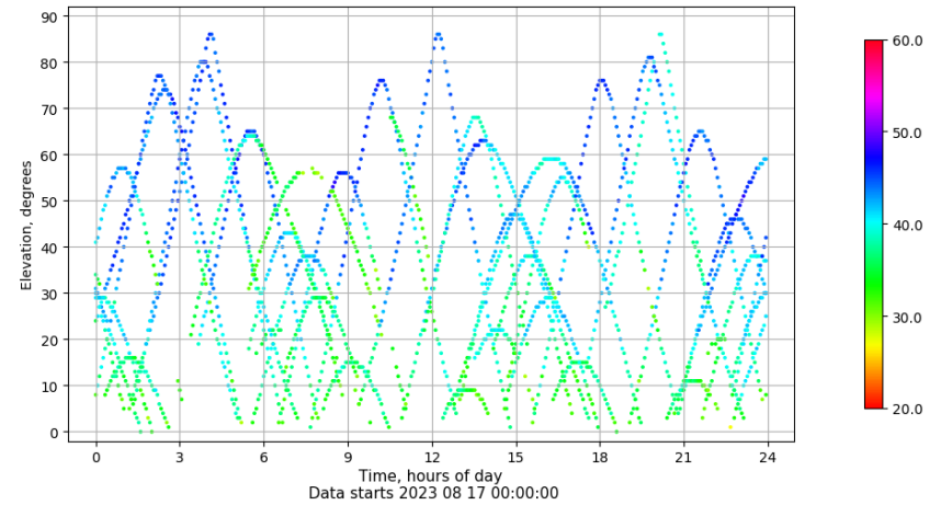
Time-elevation plot for station ALC1. Signal to Noise S1C Data file ALC100ESP_R_2023229.xtr
