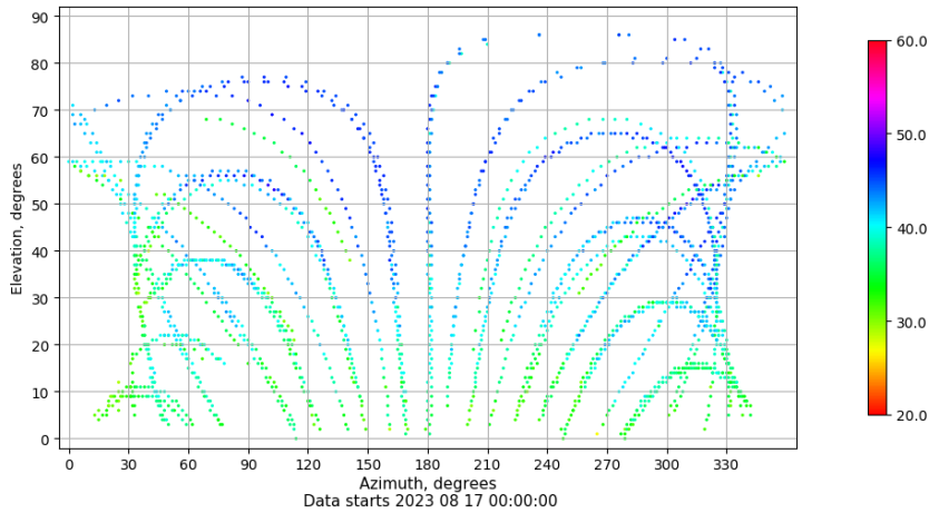
Azimuth-elevation plot for station ALC1. Signal to Noise S1C Data file ALC100ESP_R_2023229.xtr
