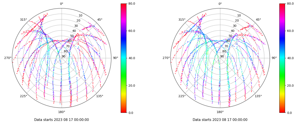
Skyplot for station ALC1. Parameter M1C Data file ALC100ESP_R_2023229.xtr Skyplot for station ALC1. Parameter M2C Data file ALC100ESP_R_2023229.xtr
