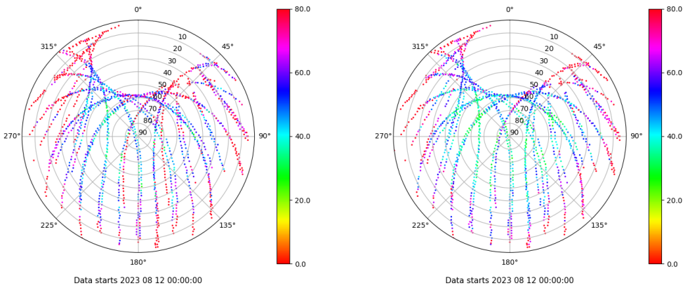
Skyplot for station ALC1. Parameter M1C Data file ALC100ESP_R_2023224.xtr Skyplot for station ALC1. Parameter M2C Data file ALC100ESP_R_2023224.xtr
