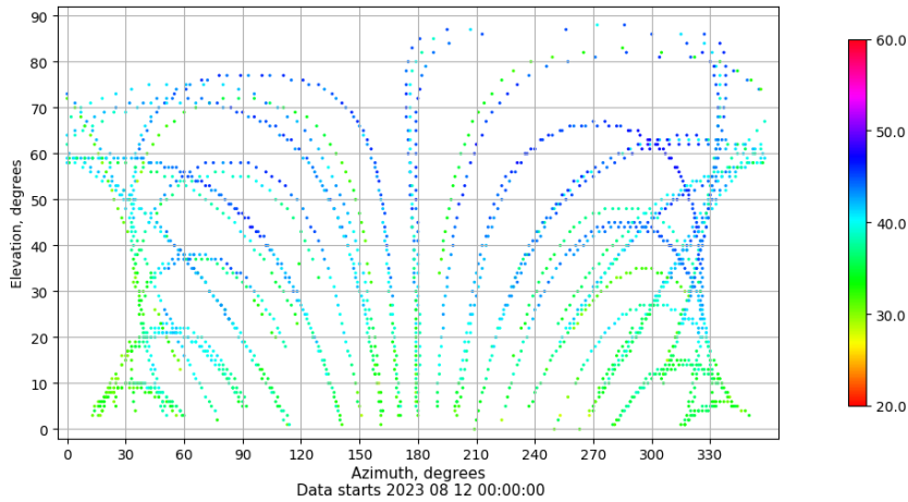
Azimuth-elevation plot for station ALC1. Signal to Noise S1C Data file ALC100ESP_R_2023224.xtr
