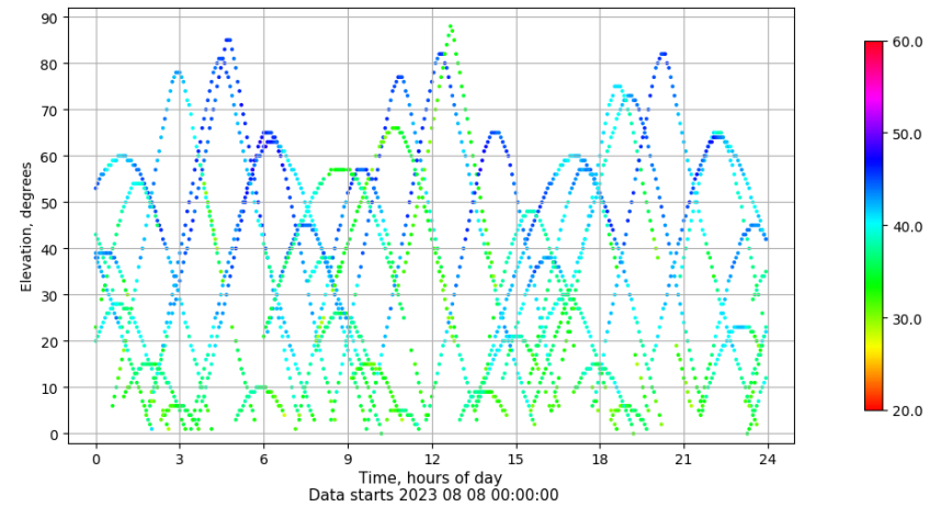
Time-elevation plot for station ALC1. Signal to Noise S1C Data file ALC100ESP_R_2023220.xtr
