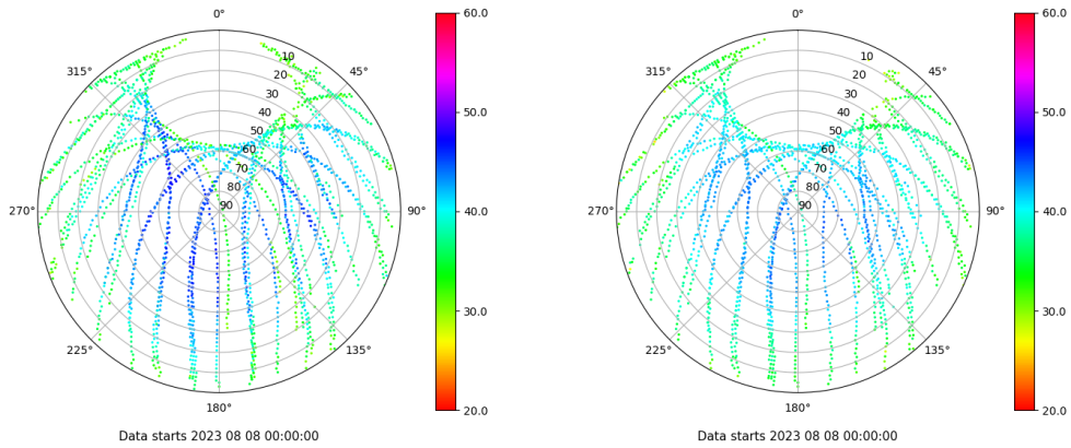
Skyplot for station ALC1. Signal to Noise S1C Data file ALC100ESP_R_2023220.xtr Skyplot for station ALC1. Signal to Noise S2C Data file ALC100ESP_R_2023220.xtr
