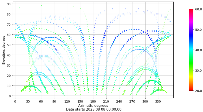
Azimuth-elevation plot for station ALC1. Signal to Noise S1C Data file ALC100ESP_R_2023220.xtr
