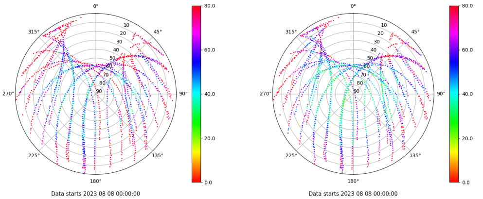
Skyplot for station ALC1. Parameter M1C Data file ALC100ESP_R_2023220.xtr Skyplot for station ALC1. Parameter M2C Data file ALC100ESP_R_2023220.xtr
