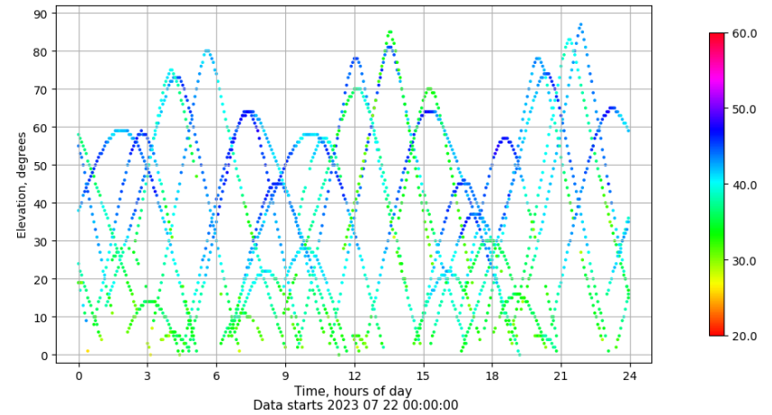
Time-elevation plot for station ALC1. Signal to Noise S1C Data file ALC100ESP_R_2023203.xtr
