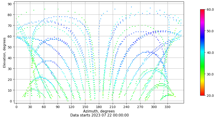
Azimuth-elevation plot for station ALC1. Signal to Noise S1C Data file ALC100ESP_R_2023203.xtr
