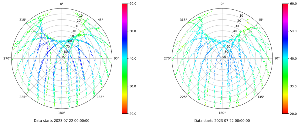
Skyplot for station ALC1. Signal to Noise S1C Data file ALC100ESP_R_2023203.xtr Skyplot for station ALC1. Signal to Noise S2C Data file ALC100ESP_R_2023203.xtr
