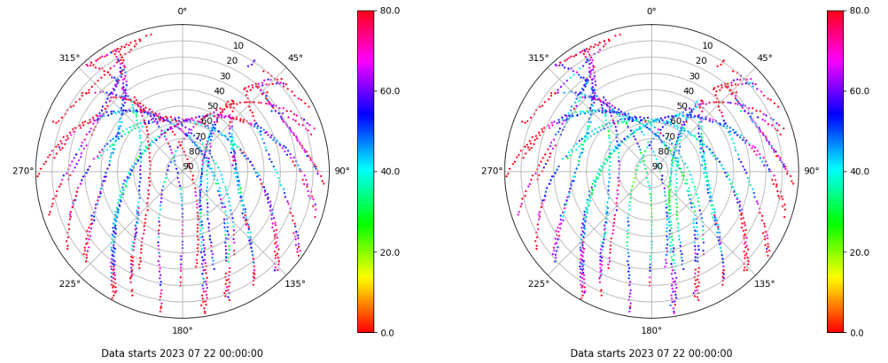
Skyplot for station ALC1. Parameter M1C Data file ALC100ESP_R_2023203.xtr Skyplot for station ALC1. Parameter M2C Data file ALC100ESP_R_2023203.xtr
