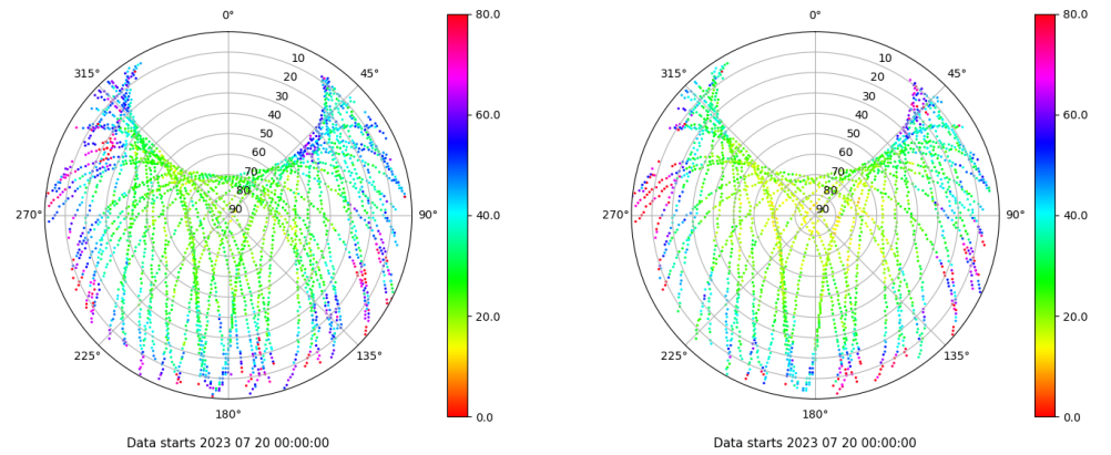
Skyplot for station ALC1. Parameter M1C Data file ALC100ESP_R_2023201.xtr Skyplot for station ALC1. Parameter M2X Data file ALC100ESP_R_2023201.xtr
