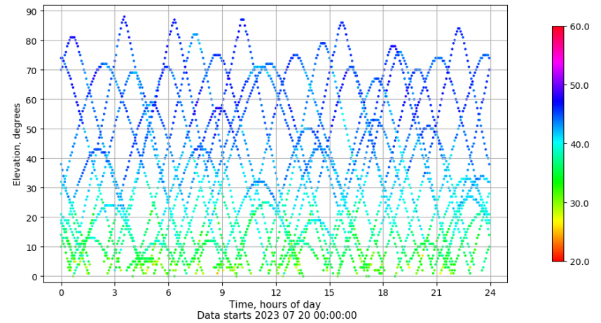
Time-elevation plot for station ALC1. Signal to Noise S1C Data file ALC100ESP_R_2023201.xtr
