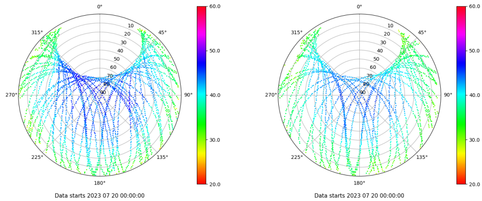
Skyplot for station ALC1. Signal to Noise S1C Data file ALC100ESP_R_2023201.xtr Skyplot for station ALC1. Signal to Noise S2X Data file ALC100ESP_R_2023201.xtr
