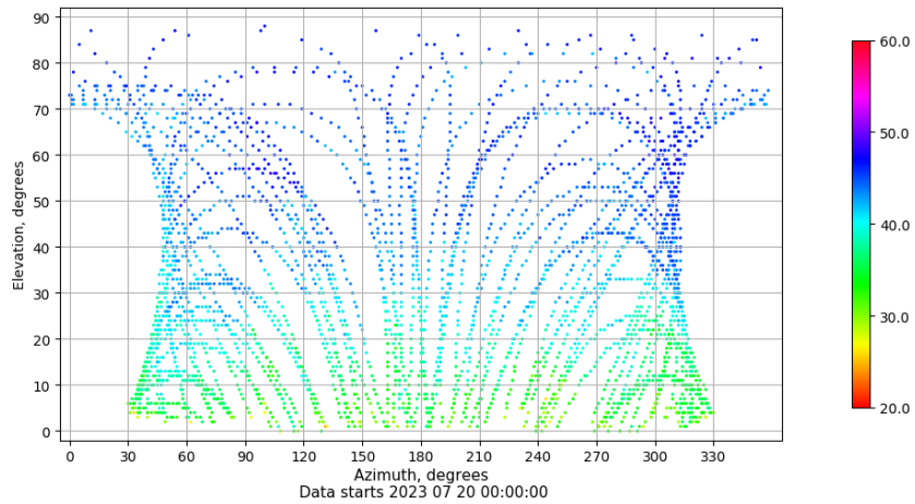
Azimuth-elevation plot for station ALC1. Signal to Noise S1C Data file ALC100ESP_R_2023201.xtr
