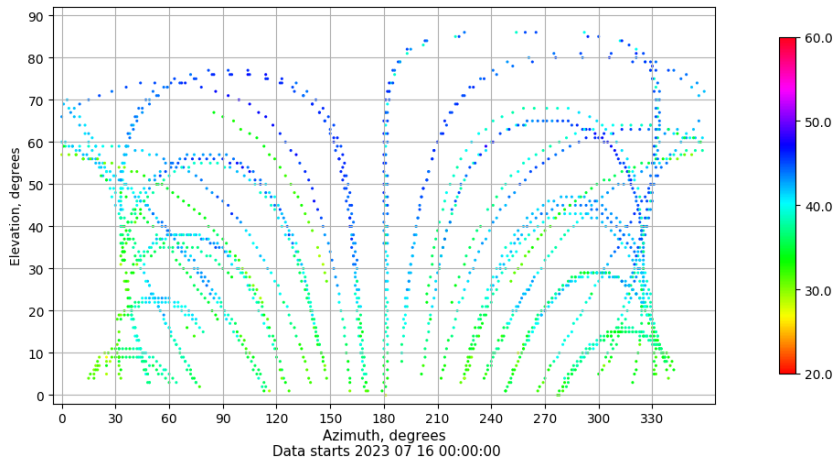
Azimuth-elevation plot for station ALC1. Signal to Noise S1C Data file ALC100ESP_R_2023197.xtr
