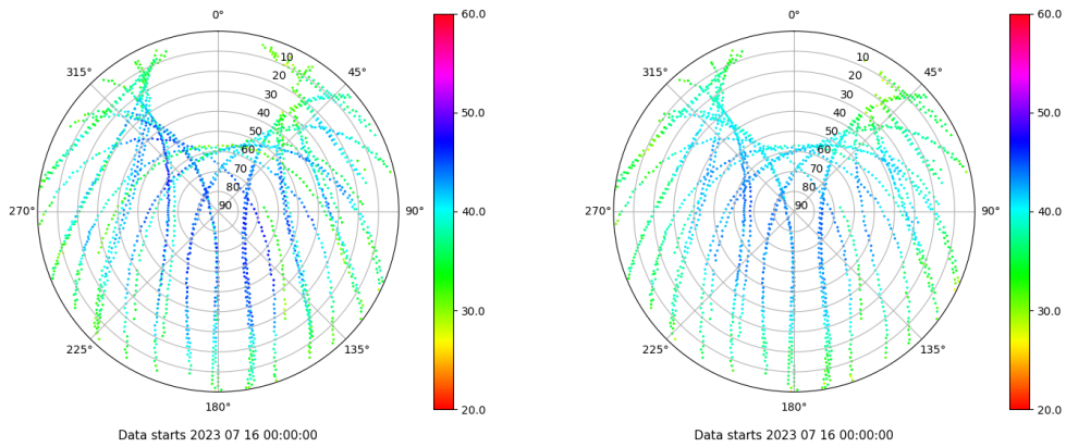
Skyplot for station ALC1. Signal to Noise S1C Data file ALC100ESP_R_2023197.xtr Skyplot for station ALC1. Signal to Noise S2C Data file ALC100ESP_R_2023197.xtr
