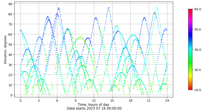
Time-elevation plot for station ALC1. Signal to Noise S1C Data file ALC100ESP_R_2023197.xtr
