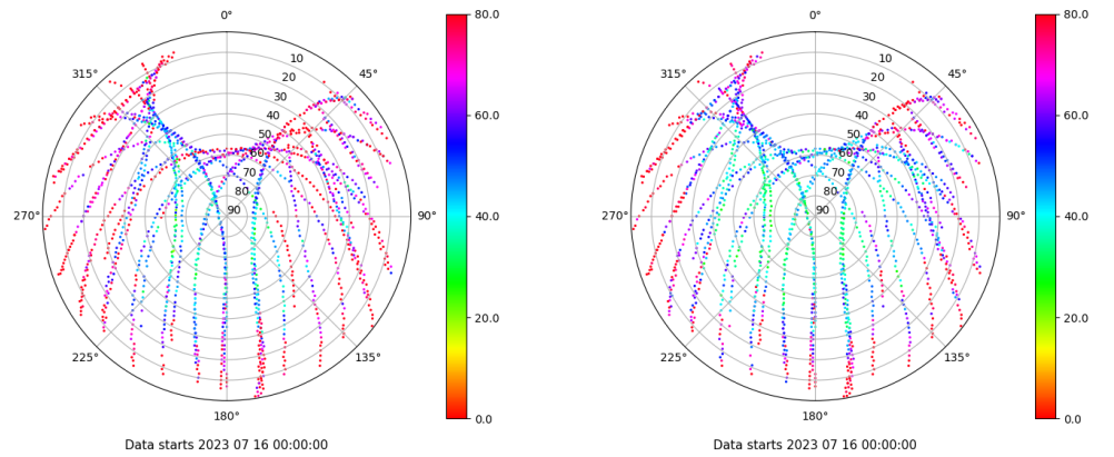
Skyplot for station ALC1. Parameter M1C Data file ALC100ESP_R_2023197.xtr Skyplot for station ALC1. Parameter M2C Data file ALC100ESP_R_2023197.xtr
