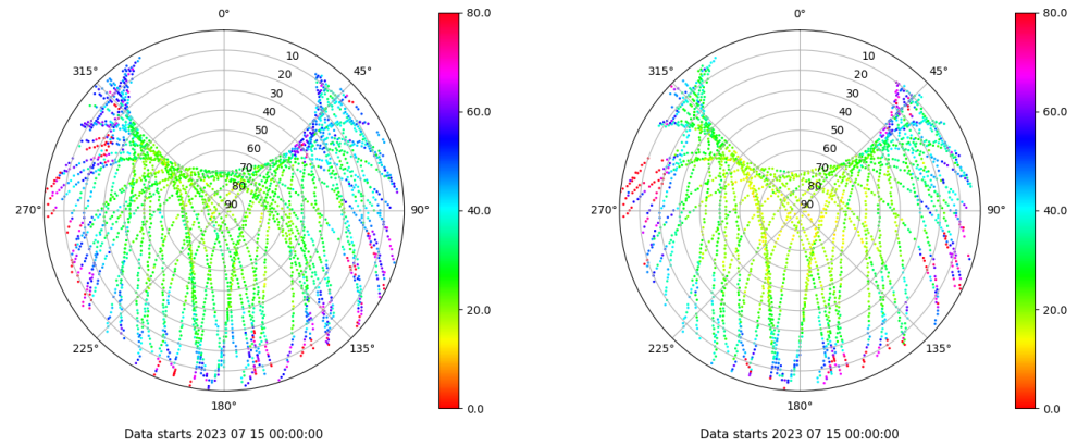
Skyplot for station ALC1. Parameter M1C Data file ALC100ESP_R_2023196.xtr Skyplot for station ALC1. Parameter M2X Data file ALC100ESP_R_2023196.xtr
