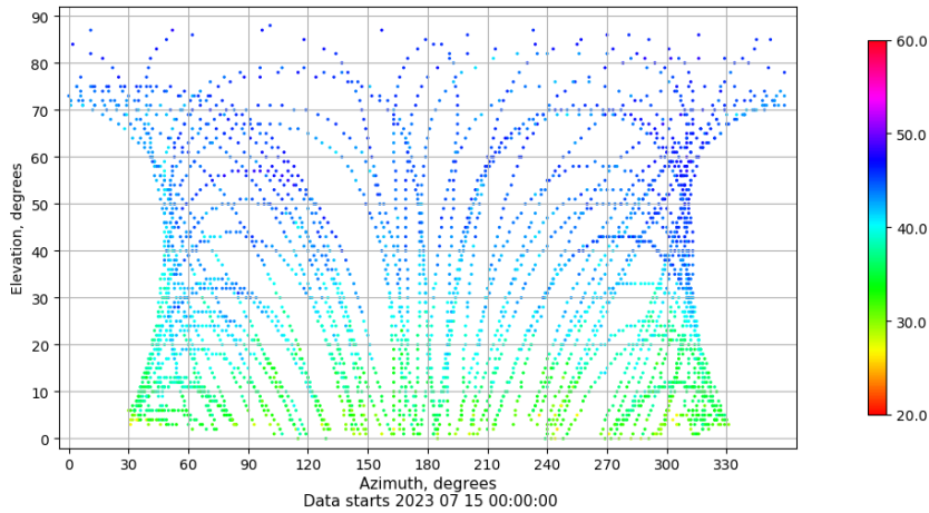
Azimuth-elevation plot for station ALC1. Signal to Noise S1C Data file ALC100ESP_R_2023196.xtr
