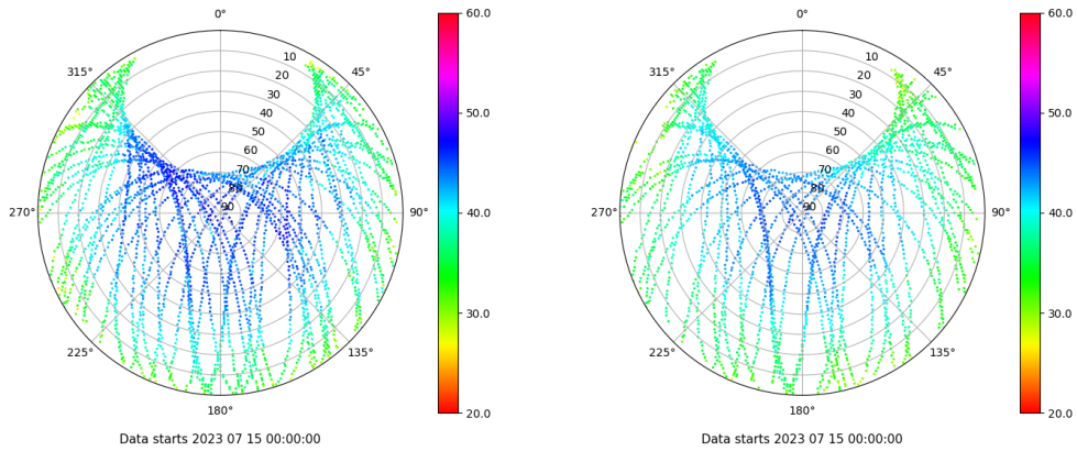
Skyplot for station ALC1. Signal to Noise S1C Data file ALC100ESP_R_2023196.xtr Skyplot for station ALC1. Signal to Noise S2X Data file ALC100ESP_R_2023196.xtr
