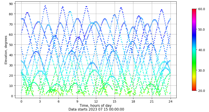
Time-elevation plot for station ALC1. Signal to Noise S1C Data file ALC100ESP_R_2023196.xtr
