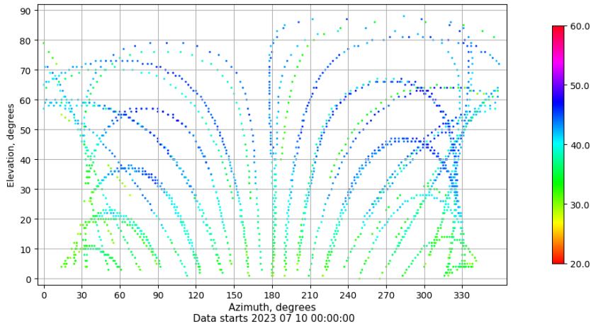
Azimuth-elevation plot for station ALC1. Signal to Noise S1C Data file ALC100ESP_R_2023191.xtr
