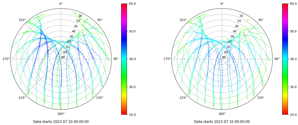
Skyplot for station ALC1. Signal to Noise S1C Data file ALC100ESP_R_2023191.xtr Skyplot for station ALC1. Signal to Noise S2C Data file ALC100ESP_R_2023191.xtr
