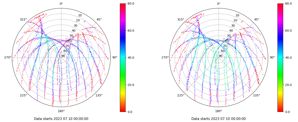
Skyplot for station ALC1. Parameter M1C Data file ALC100ESP_R_2023191.xtr Skyplot for station ALC1. Parameter M2C Data file ALC100ESP_R_2023191.xtr
