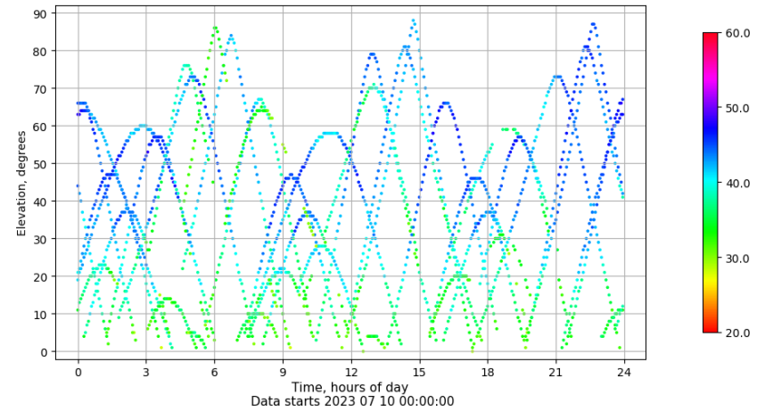
Time-elevation plot for station ALC1. Signal to Noise S1C Data file ALC100ESP_R_2023191.xtr
