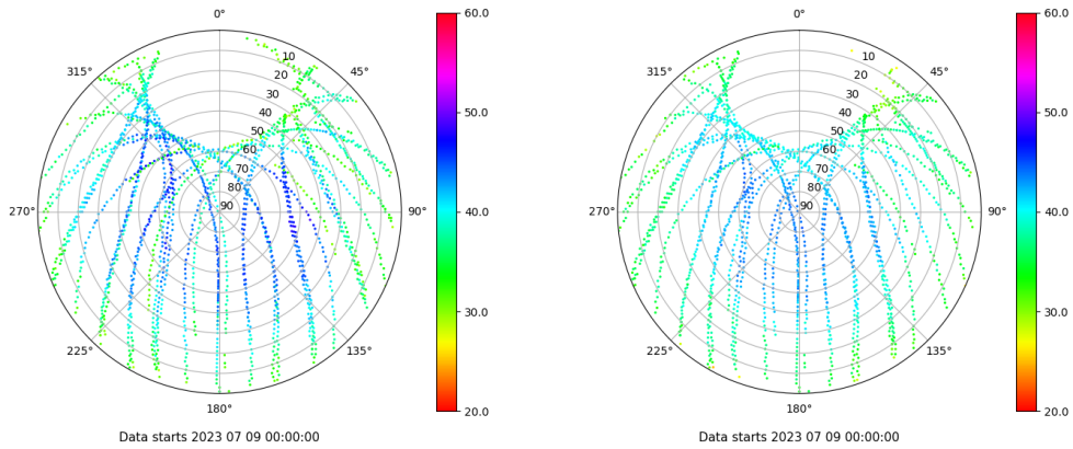
Skyplot for station ALC1. Signal to Noise S1C Data file ALC100ESP_R_2023190.xtr Skyplot for station ALC1. Signal to Noise S2C Data file ALC100ESP_R_2023190.xtr
