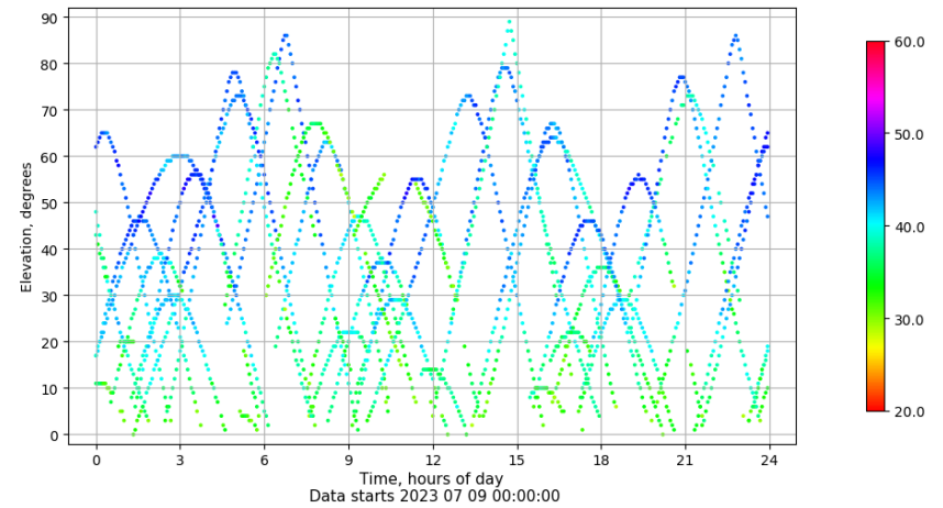
Time-elevation plot for station ALC1. Signal to Noise S1C Data file ALC100ESP_R_2023190.xtr
