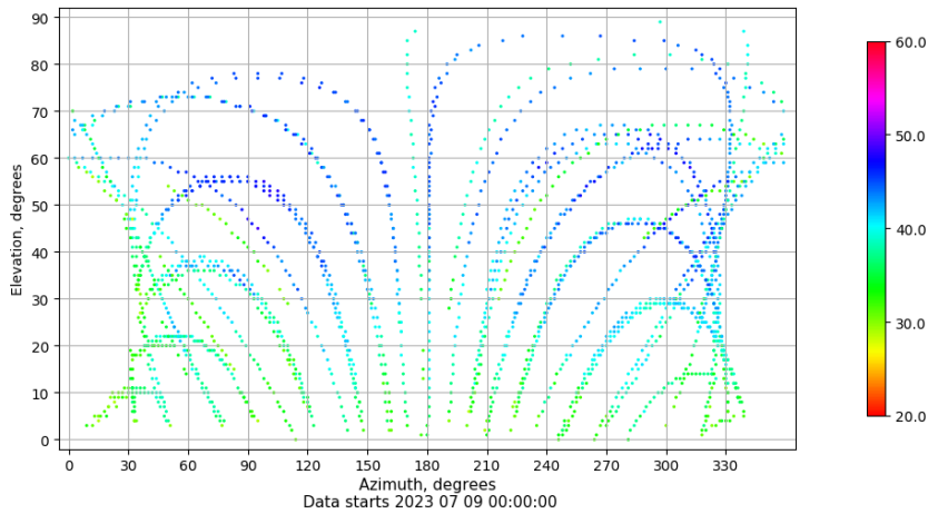
Azimuth-elevation plot for station ALC1. Signal to Noise S1C Data file ALC100ESP_R_2023190.xtr
