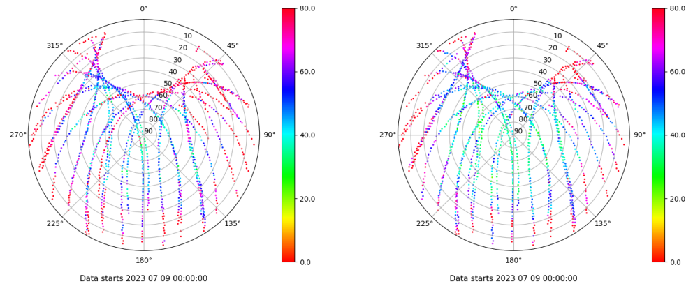
Skyplot for station ALC1. Parameter M1C Data file ALC100ESP_R_2023190.xtr Skyplot for station ALC1. Parameter M2C Data file ALC100ESP_R_2023190.xtr
