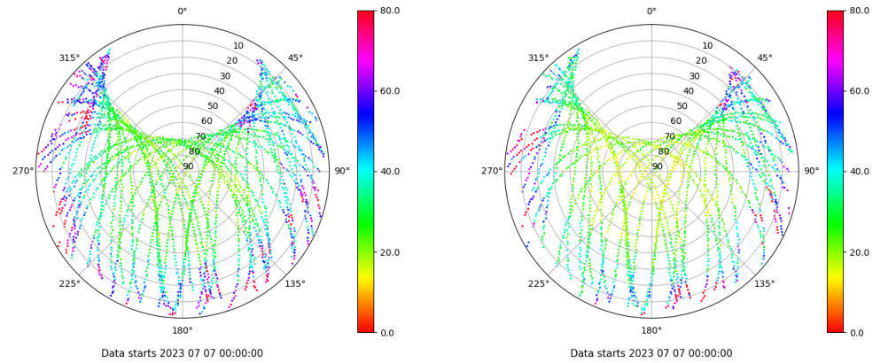
Skyplot for station ALC1. Parameter M1C Data file ALC100ESP_R_2023188.xtr Skyplot for station ALC1. Parameter M2X Data file ALC100ESP_R_2023188.xtr
