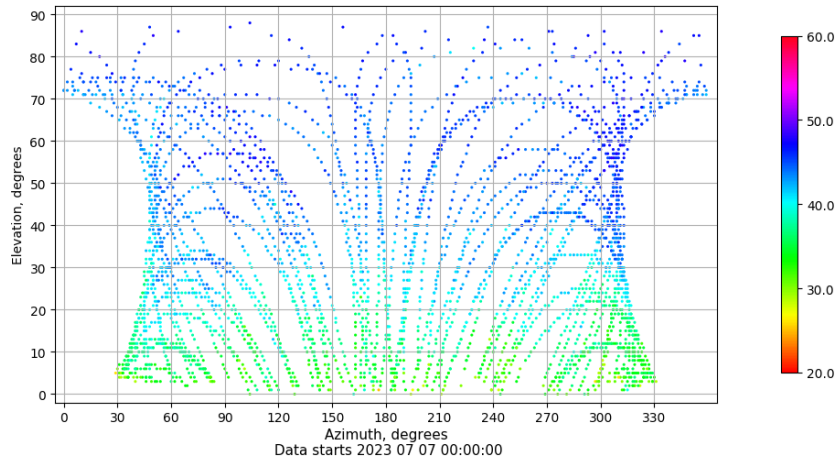
Azimuth-elevation plot for station ALC1. Signal to Noise S1C Data file ALC100ESP_R_2023188.xtr
