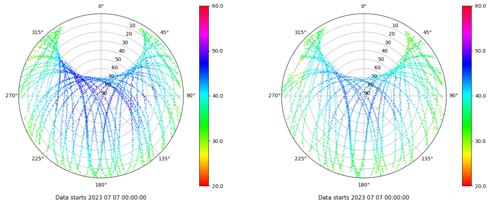
Skyplot for station ALC1. Signal to Noise S1C Data file ALC100ESP_R_2023188.xtr Skyplot for station ALC1. Signal to Noise S2X Data file ALC100ESP_R_2023188.xtr
