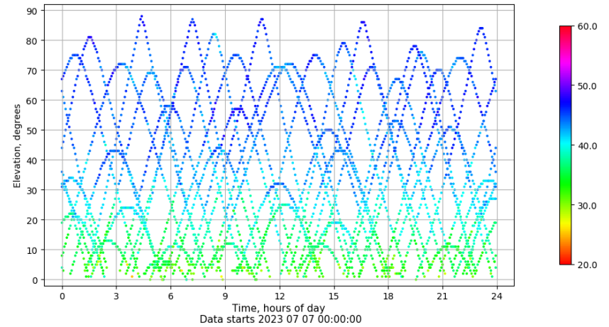
Time-elevation plot for station ALC1. Signal to Noise S1C Data file ALC100ESP_R_2023188.xtr
