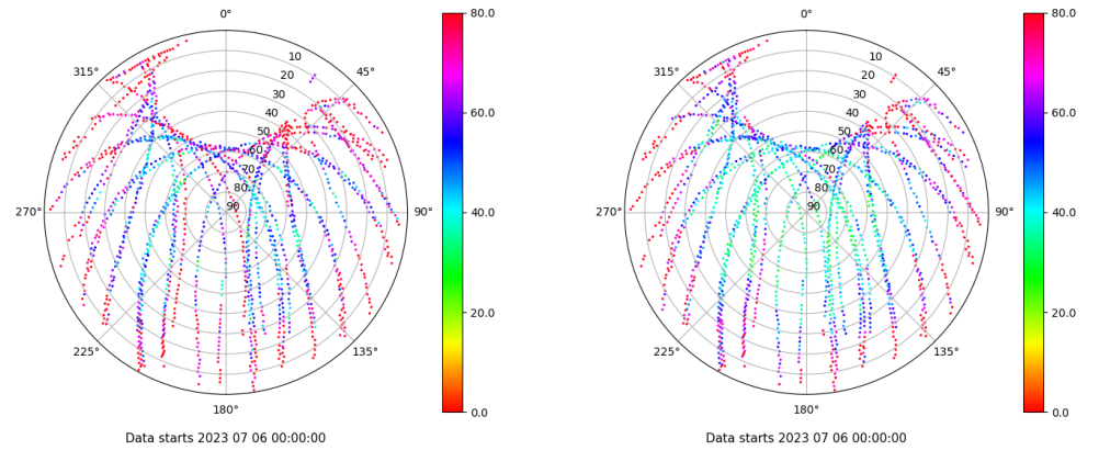
Skyplot for station ALC1. Parameter M1C Data file ALC100ESP_R_2023187.xtr Skyplot for station ALC1. Parameter M2C Data file ALC100ESP_R_2023187.xtr
