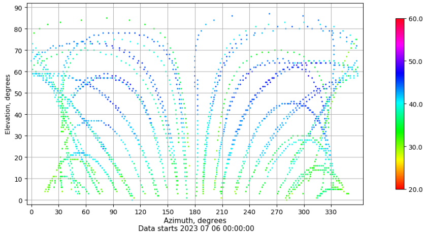
Azimuth-elevation plot for station ALC1. Signal to Noise S1C Data file ALC100ESP_R_2023187.xtr
