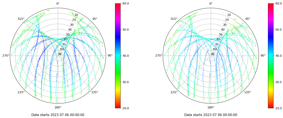
Skyplot for station ALC1. Signal to Noise S1C Data file ALC100ESP_R_2023187.xtr Skyplot for station ALC1. Signal to Noise S2C Data file ALC100ESP_R_2023187.xtr
