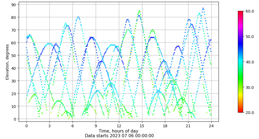
Time-elevation plot for station ALC1. Signal to Noise S1C Data file ALC100ESP_R_2023187.xtr
