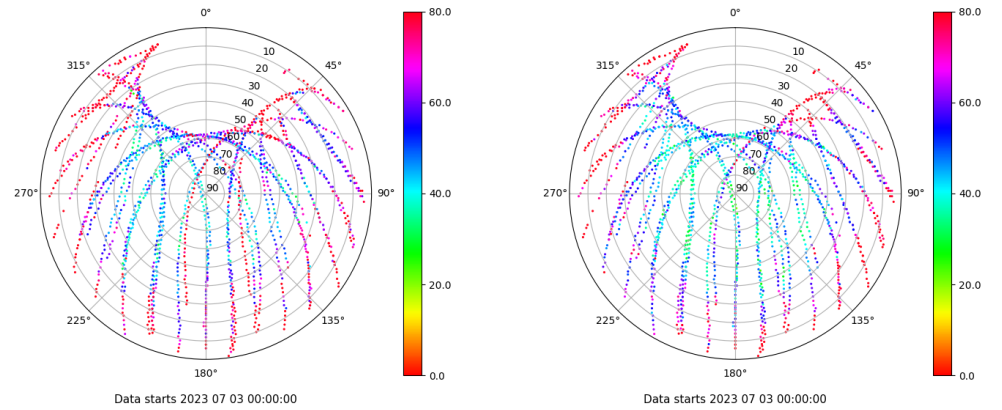
Skyplot for station ALC1. Parameter M1C Data file ALC100ESP_R_2023184.xtr Skyplot for station ALC1. Parameter M2C Data file ALC100ESP_R_2023184.xtr
