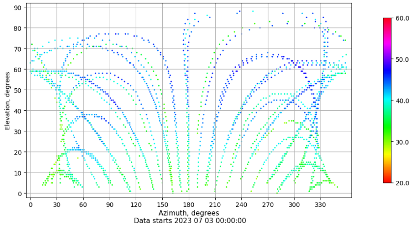
Azimuth-elevation plot for station ALC1. Signal to Noise S1C Data file ALC100ESP_R_2023184.xtr
