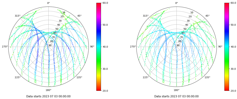
Skyplot for station ALC1. Signal to Noise S1C Data file ALC100ESP_R_2023184.xtr Skyplot for station ALC1. Signal to Noise S2C Data file ALC100ESP_R_2023184.xtr
