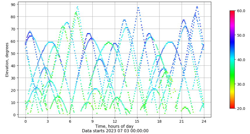
Time-elevation plot for station ALC1. Signal to Noise S1C Data file ALC100ESP_R_2023184.xtr
