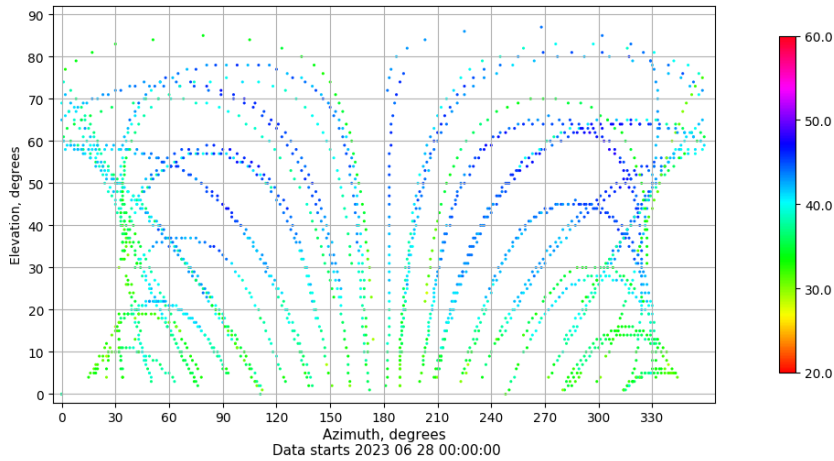
Azimuth-elevation plot for station ALC1. Signal to Noise S1C Data file ALC100ESP_R_2023179.xtr
