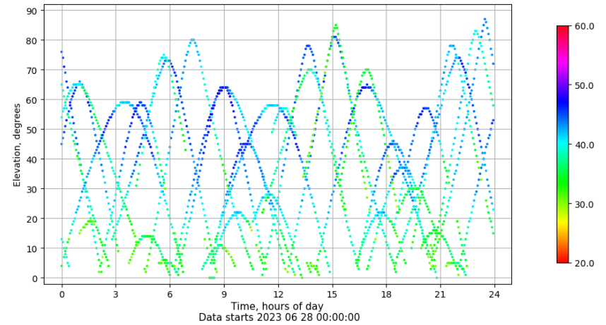
Time-elevation plot for station ALC1. Signal to Noise S1C Data file ALC100ESP_R_2023179.xtr
