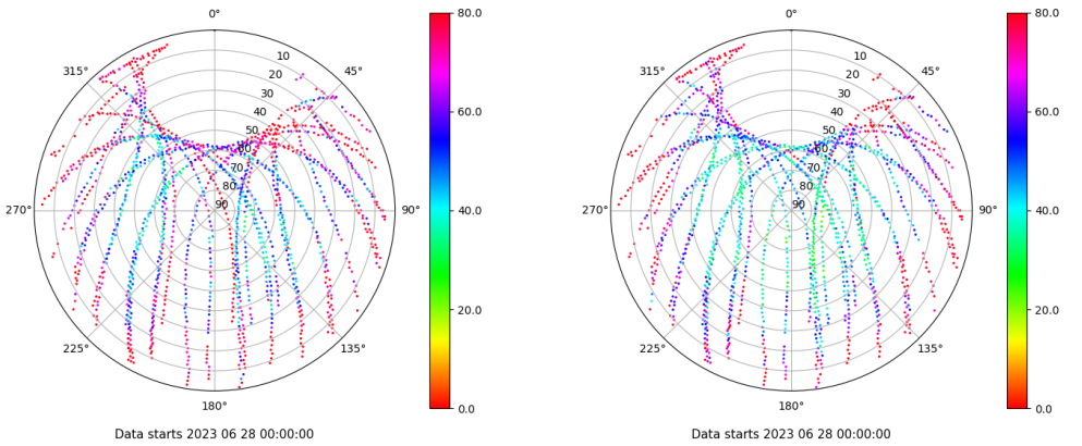
Skyplot for station ALC1. Parameter M1C Data file ALC100ESP_R_2023179.xtr Skyplot for station ALC1. Parameter M2C Data file ALC100ESP_R_2023179.xtr
