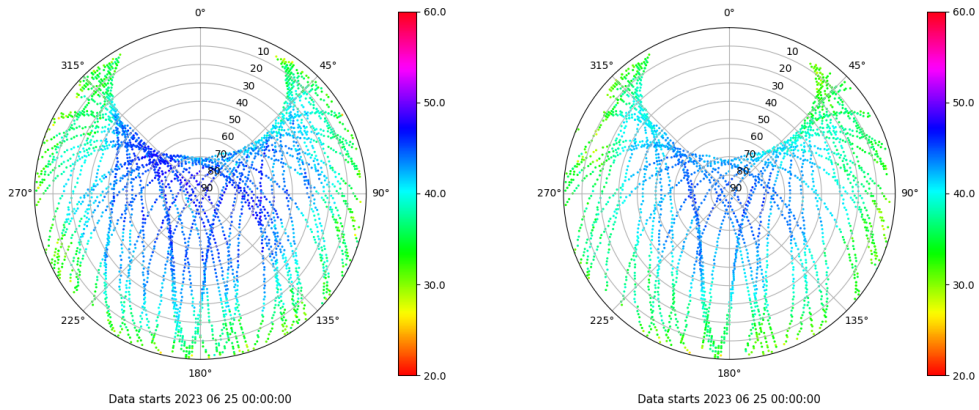
Skyplot for station ALC1. Signal to Noise S1C Data file ALC100ESP_R_2023176.xtr Skyplot for station ALC1. Signal to Noise S2X Data file ALC100ESP_R_2023176.xtr
