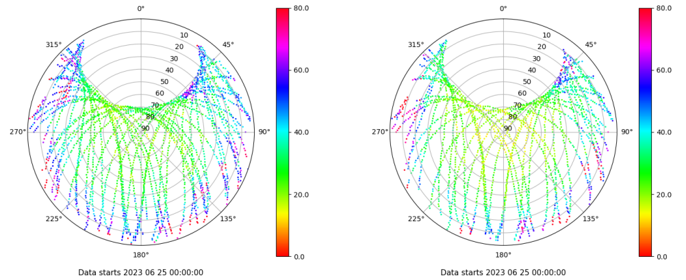
Skyplot for station ALC1. Parameter M1C Data file ALC100ESP_R_2023176.xtr Skyplot for station ALC1. Parameter M2X Data file ALC100ESP_R_2023176.xtr
