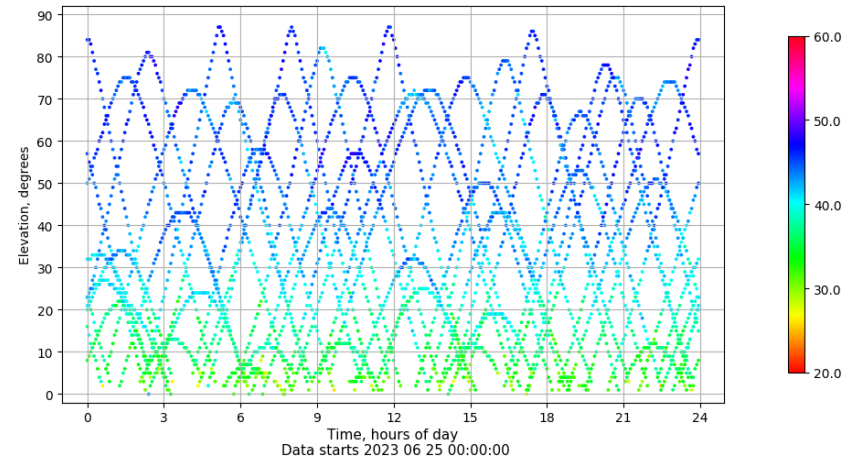
Time-elevation plot for station ALC1. Signal to Noise S1C Data file ALC100ESP_R_2023176.xtr
