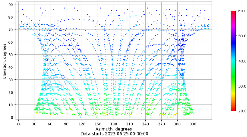
Azimuth-elevation plot for station ALC1. Signal to Noise S1C Data file ALC100ESP_R_2023176.xtr
