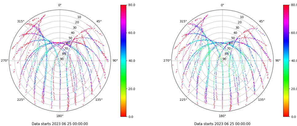
Skyplot for station ALC1. Parameter M1C Data file ALC100ESP_R_2023176.xtr Skyplot for station ALC1. Parameter M2C Data file ALC100ESP_R_2023176.xtr
