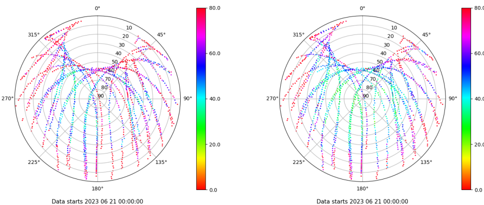
Skyplot for station ALC1. Parameter M1C Data file ALC100ESP_R_2023172.xtr Skyplot for station ALC1. Parameter M2C Data file ALC100ESP_R_2023172.xtr
