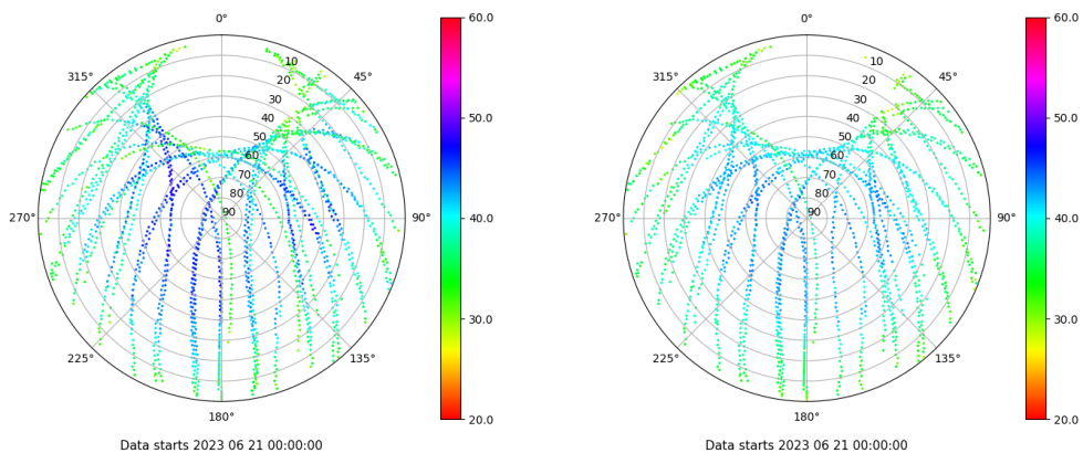
Skyplot for station ALC1. Signal to Noise S1C Data file ALC100ESP_R_2023172.xtr Skyplot for station ALC1. Signal to Noise S2C Data file ALC100ESP_R_2023172.xtr
