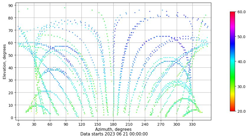
Azimuth-elevation plot for station ALC1. Signal to Noise S1C Data file ALC100ESP_R_2023172.xtr
