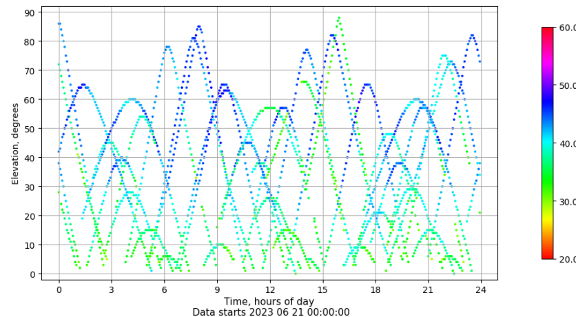
Time-elevation plot for station ALC1. Signal to Noise S1C Data file ALC100ESP_R_2023172.xtr
